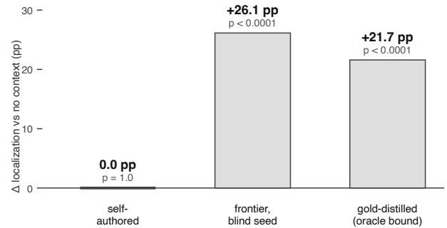
Figure 3. Paired improvement in the 8B executor's gold-file localization over its no-context control, by context author (36 pairs \times 5 repetitions). Resolve-rate deltas are not significant at this tier (oracle +2.2 pp, p = 0.22 ).
