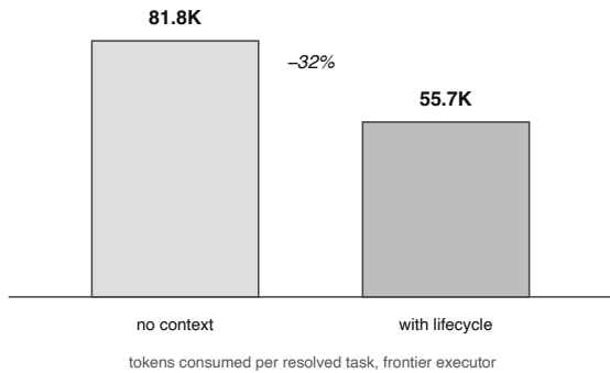
Figure 4. Total tokens spent per successfully resolved task (frontier executor, 48 episodes/arm). Successful episodes cost the same in both arms ( \approx 33.6K ); the saving comes from fewer failed explorations. The oracle-taught variant spends like the lifecycle arm (64.1K/resolved) without matching its resolve rate.
