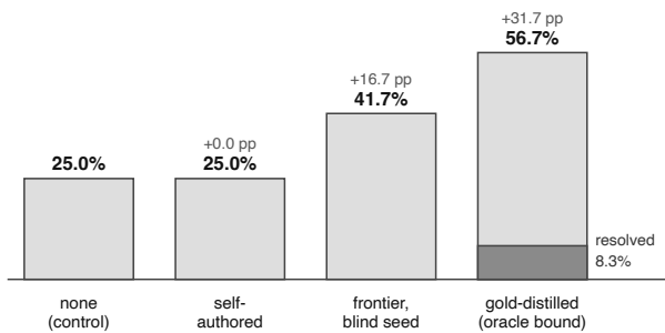
Figure 3. Gold-file localization of the 8B executor on held-out tasks, by context author (light bars); the dark segment is the oracle arm's resolve rate — the executor's only resolves in the study. Deltas vs control: self +0.0 ( p = 1.0 ), blind seed +16.7 ( p = 0.041 ), oracle +31.7 ( p = 0.0005 ).
