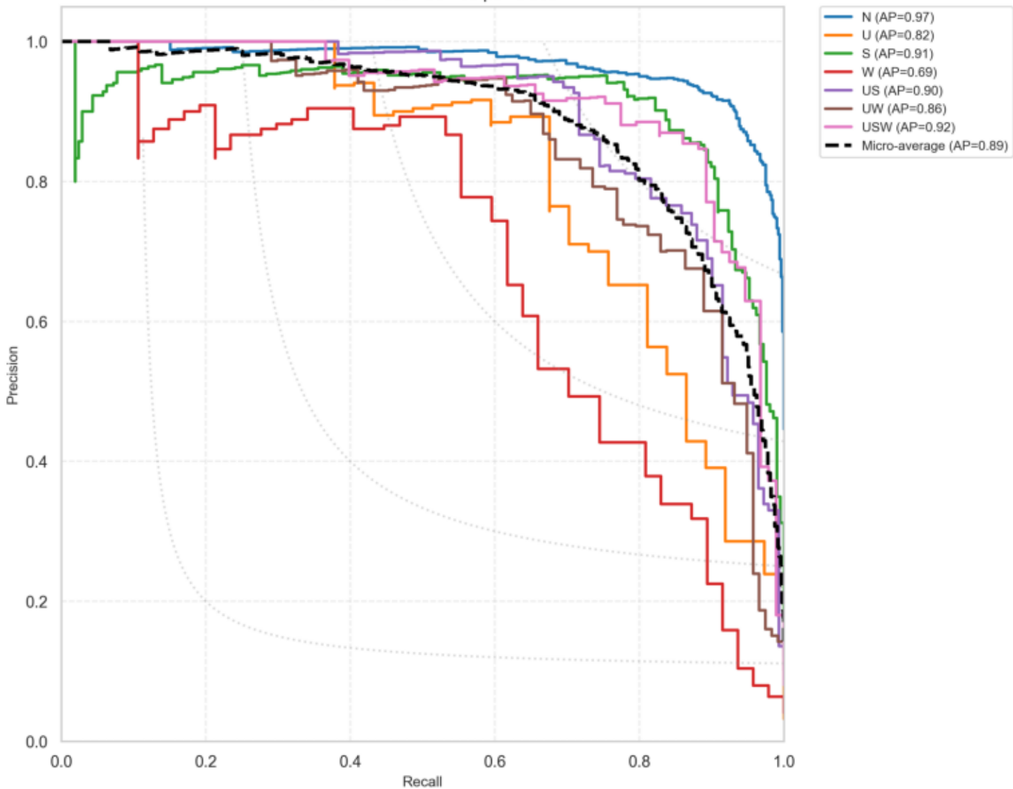
Precision–Recall Curves per Class
