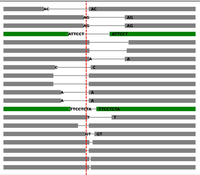
TK6 WT 4h
