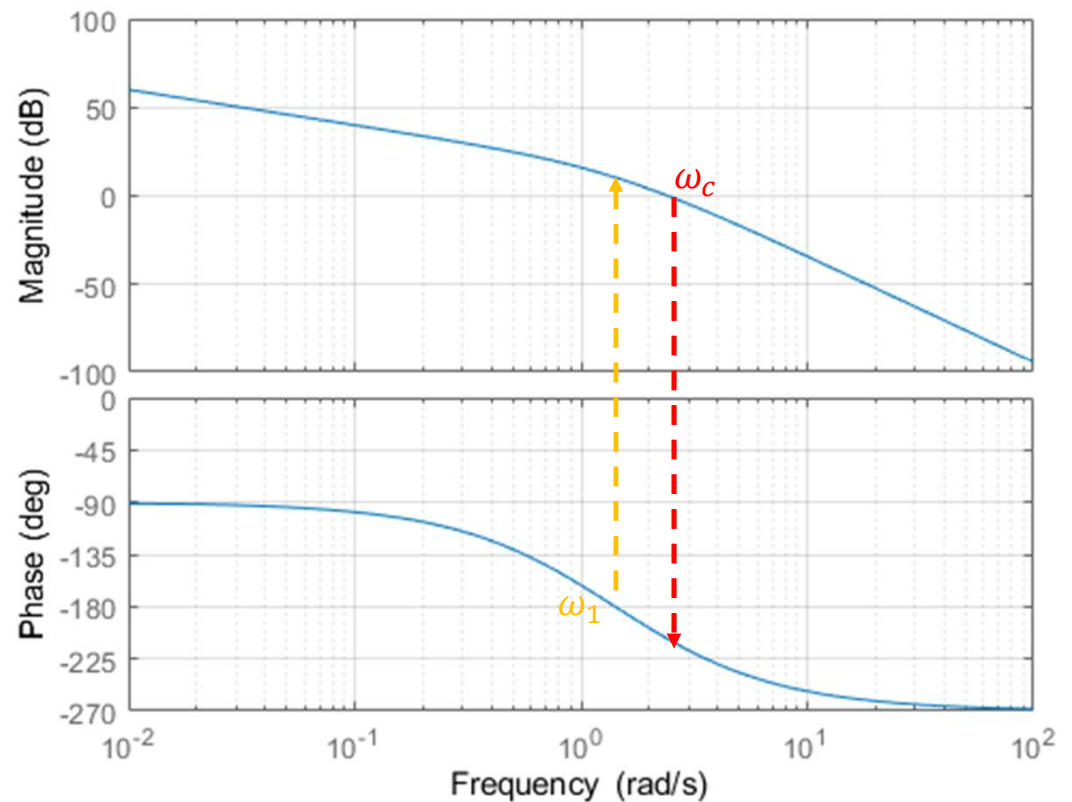
Bode Diagram
