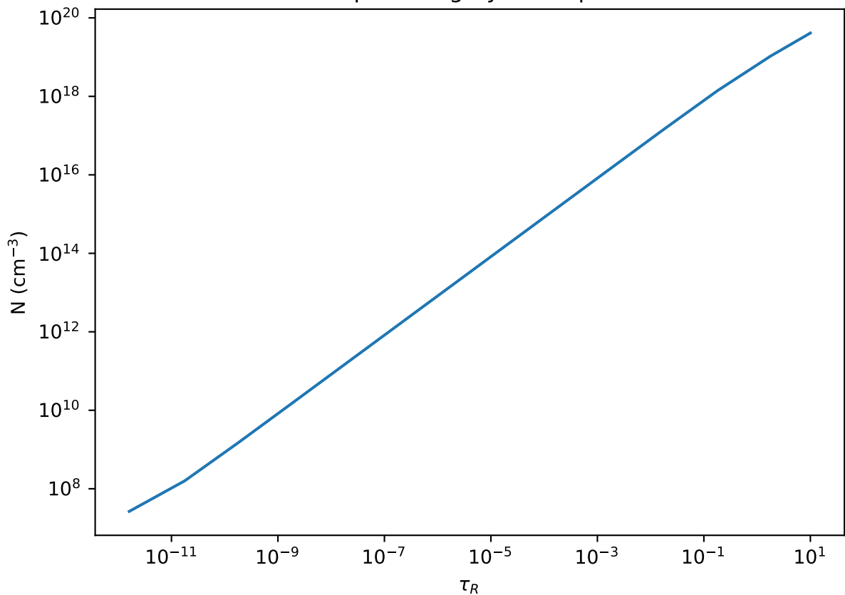
Canopus-like grey atmosphere
