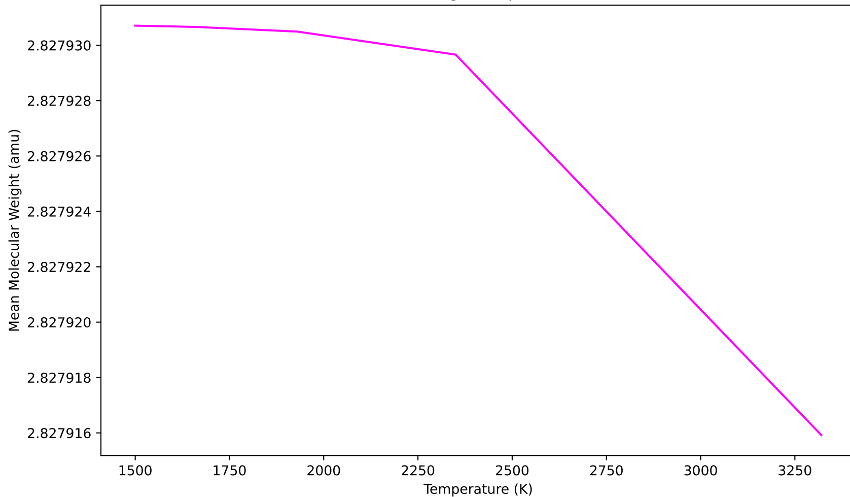
Mean Molecular Weight - Equilibrium Solve Test
