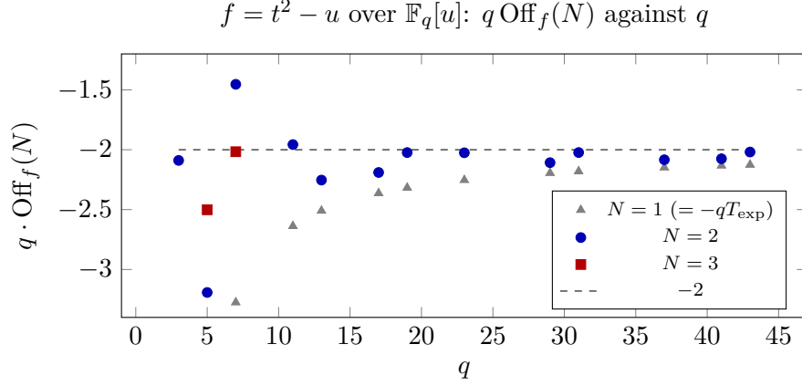
Figure 1: Exact values of q \text{Off}_f(N) for f = t^2 - u (research/paper-III/scripts/offq.ts; N = 3 needs all squarefree moduli of degree \leq 6 and was computed for q \leq 7 ). Theorem 26 gives the limit -2 for N = 1, 2 ; Conjecture 29 predicts -1 for N = 3 . The N = 1 values approach -2 from below like -2 - 5/q .
