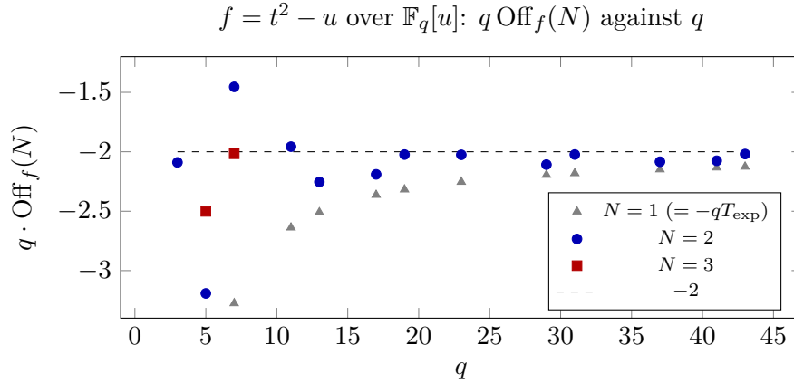
Figure 1: Exact values of q \text{Off}_f(N) for f = t^2 - u (research/paper-III/scripts/offq.ts; N = 3 needs all squarefree moduli of degree \leq 6 and was computed for q \leq 7 ). Theorem 25 gives the limit -2 for N = 1, 2 ; Conjecture 28 predicts -1 for N = 3 . The N = 1 values approach -2 from below like -2 - 5/q .
