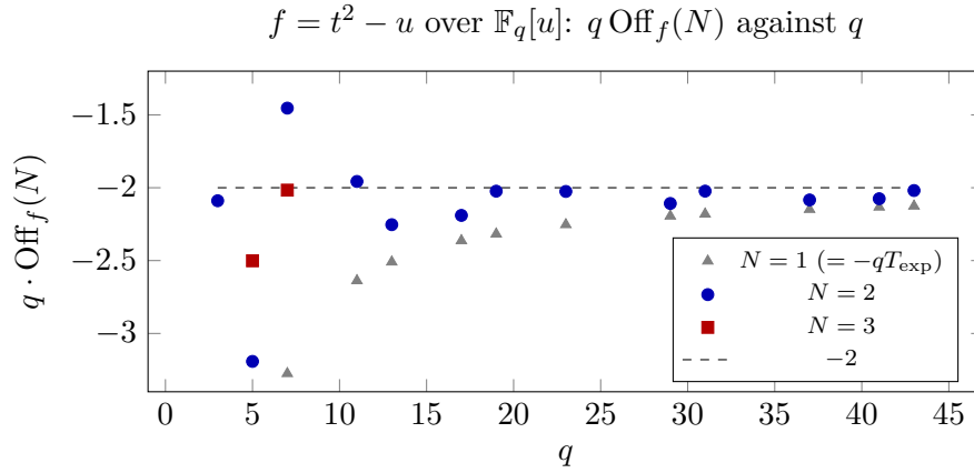
Figure 1: Exact values of q \text{ Off}_f(N) for f = t^2 - u ( research/paper-III/scripts/offq.ts ; N = 3 needs all squarefree moduli of degree \leq 6 and was computed for q \leq 7 ). Theorem 22 gives the limit -2 for N = 1, 2 ; Conjecture 25 predicts -1 for N = 3 . The N = 1 values approach -2 from below like -2 - 5/q .
