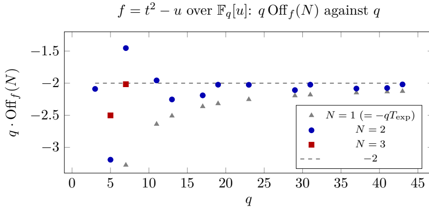
Figure 1: Exact values of q\text{Off}_f(N) for f = t^2 - u (scripts/offq.ts; N = 3 needs all squarefree moduli of degree \leq 6 and was computed for q \leq 7 ). Theorem 10 gives the limit -2 for N = 1, 2 ; Conjecture 13 predicts -1 for N = 3 . The N = 1 values approach -2 from below like -2 - 5/q .
