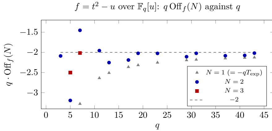
Figure 1: Exact values of q \text{Off}_f(N) for f = t^2 - u (research/paper-III/scripts/offq.ts; N = 3 needs all squarefree moduli of degree \leq 6 and was computed for q \leq 7 ). Theorem 22 gives the limit -2 for N = 1, 2 ; Conjecture 25 predicts -1 for N = 3 . The N = 1 values approach -2 from below like -2 - 5/q .
