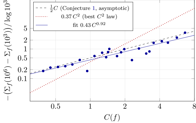
Figure 2: The exact test. For 25 quadratics the slope of \Sigma_f(H) per unit of \log H over 10^3 \leq H \leq 10^6 , computed from the closed formula of Theorem 5 with no truncation of the h -dependent part, against C(f) on logarithmic axes. A law -kC^\alpha is a straight line of slope \alpha ; the logarithmic fit gives \alpha = 0.92 \pm 0.08 (unweighted: 1.19 \pm 0.11 ). The dashed line is the conjectured asymptotic \frac{1}{2}C ; the finite- H points lie below it by the drift of the constant term (Table 2).
