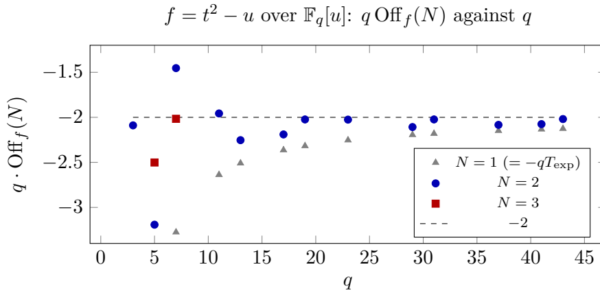
Figure 1: Exact values of q \text{Off}_f(N) for f = t^2 - u (research/paper-III/scripts/offq.ts; N = 3 needs all squarefree moduli of degree \leq 6 and was computed for q \leq 7 ). Theorem 20 gives the limit -2 for N = 1, 2 ; Conjecture 23 predicts -1 for N = 3 . The N = 1 values approach -2 from below like -2 - 5/q .
