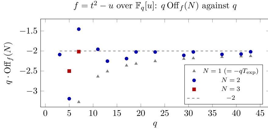
Figure 1: Exact values of q \text{Off}_f(N) for f = t^2 - u (research/paper-III/scripts/offq.ts; N = 3 needs all squarefree moduli of degree \leq 6 and was computed for q \leq 7 ). Theorem 20 gives the limit -2 for N = 1, 2 ; Conjecture 23 predicts -1 for N = 3 . The N = 1 values approach -2 from below like -2 - 5/q .
