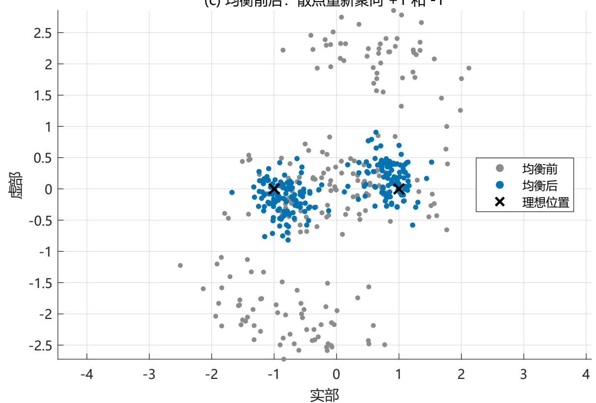
(c) 均衡前后：散点重新聚向 +1 和 -1
