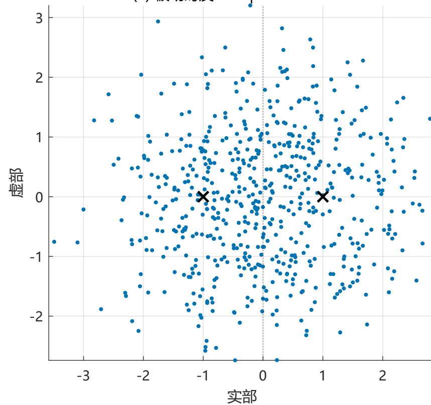
(e) 被动时反 DFE | BER = 0.6817
