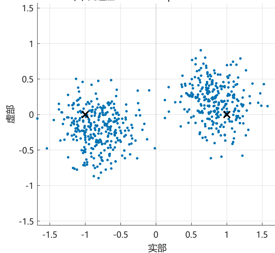
(e) 被动时反 DFE | BER = 0.6817
