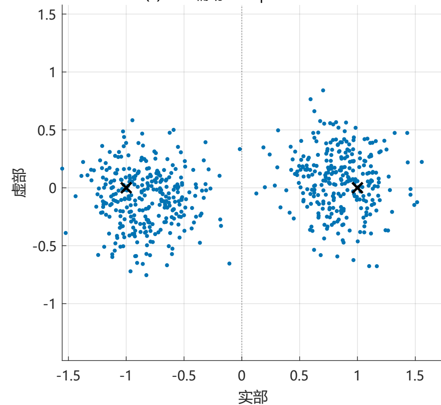
(f) 子带被动时反 DFE | BER = 0.5583
