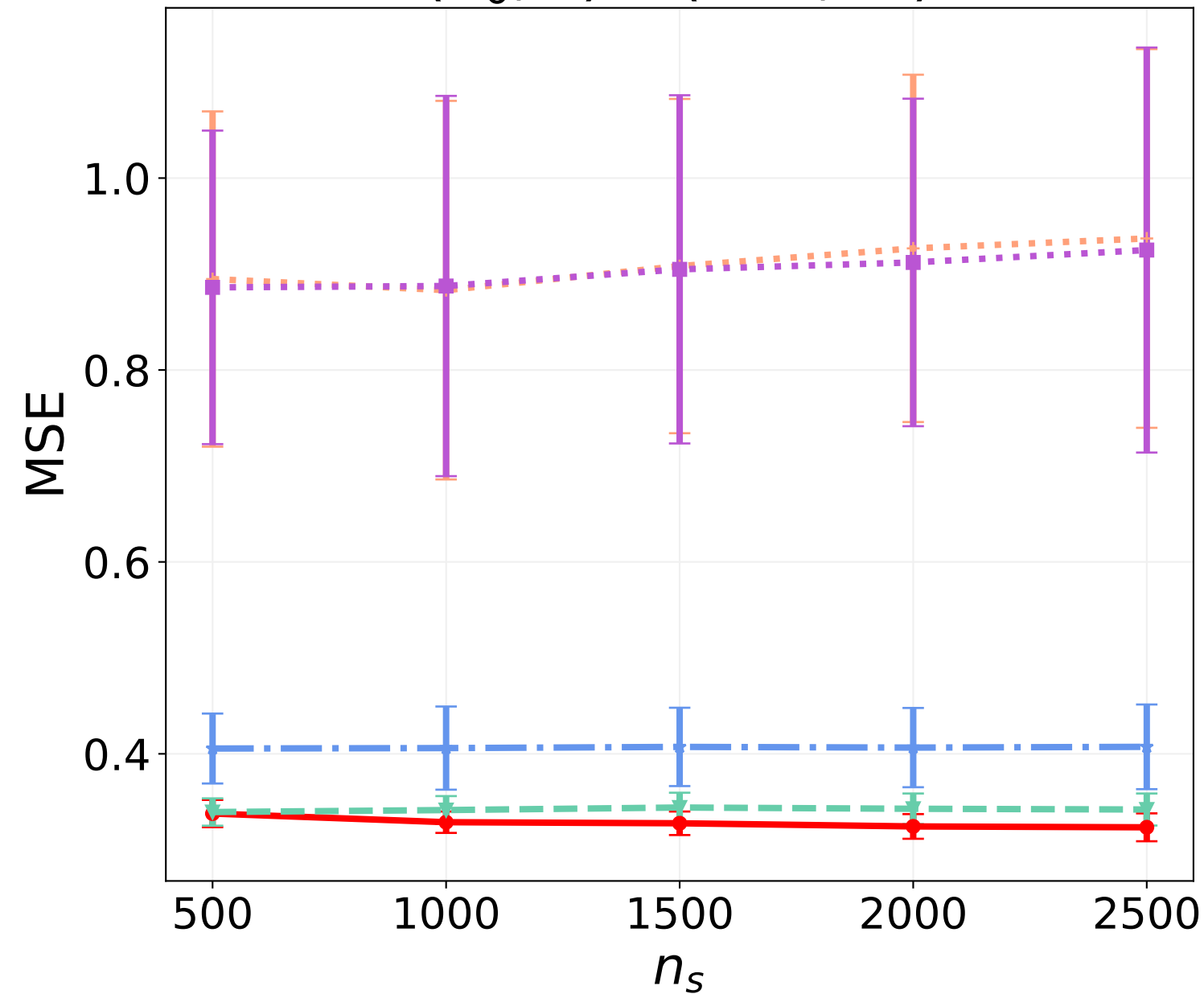
(n_0, d) = (500, 10)
