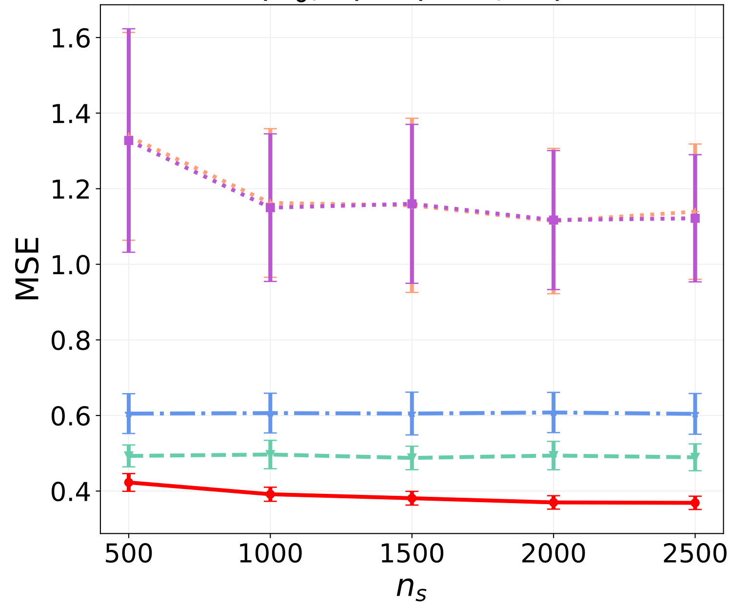
(n_0, d) = (500, 20)
