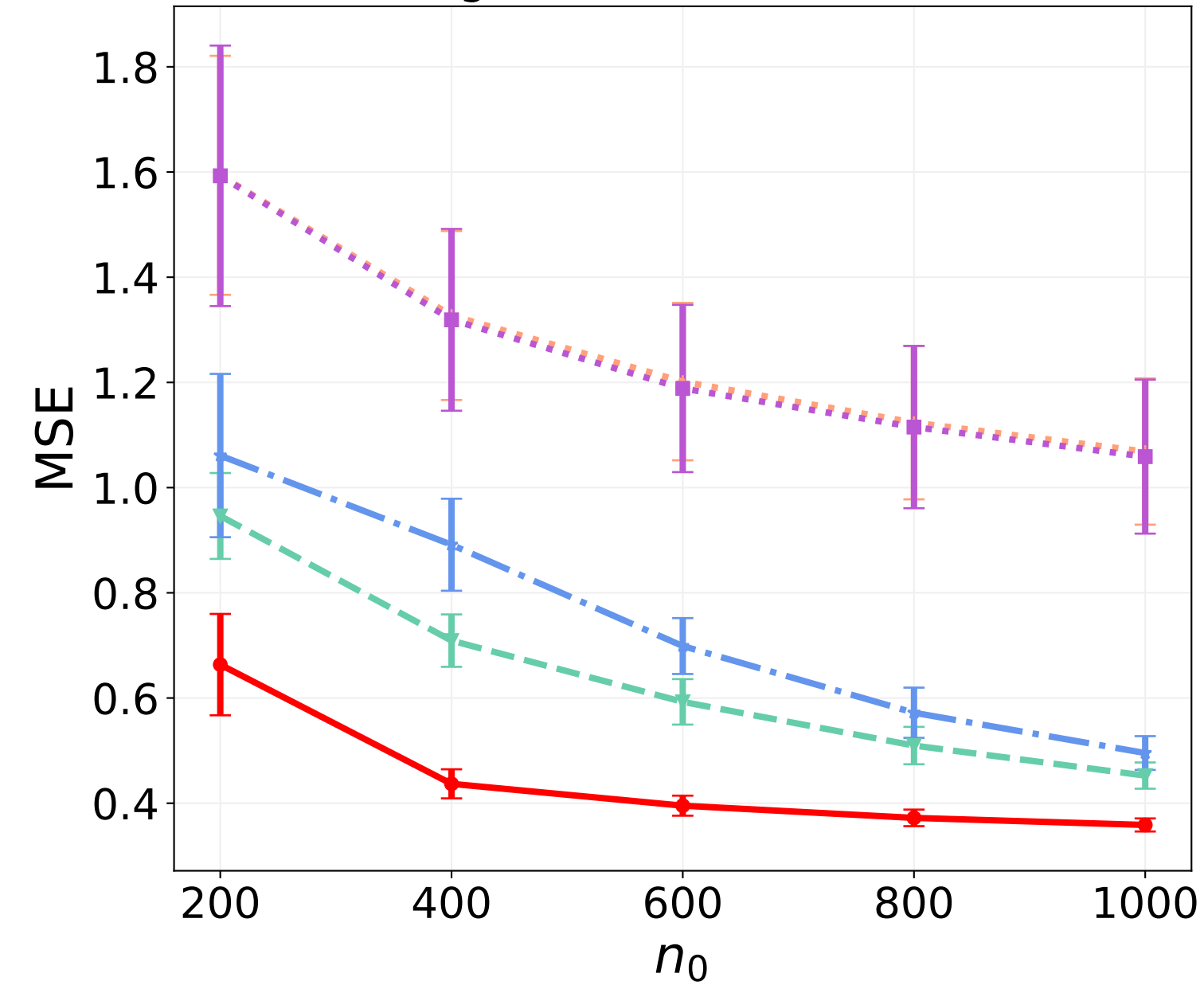
(n_s, d) = (2000, 30)
