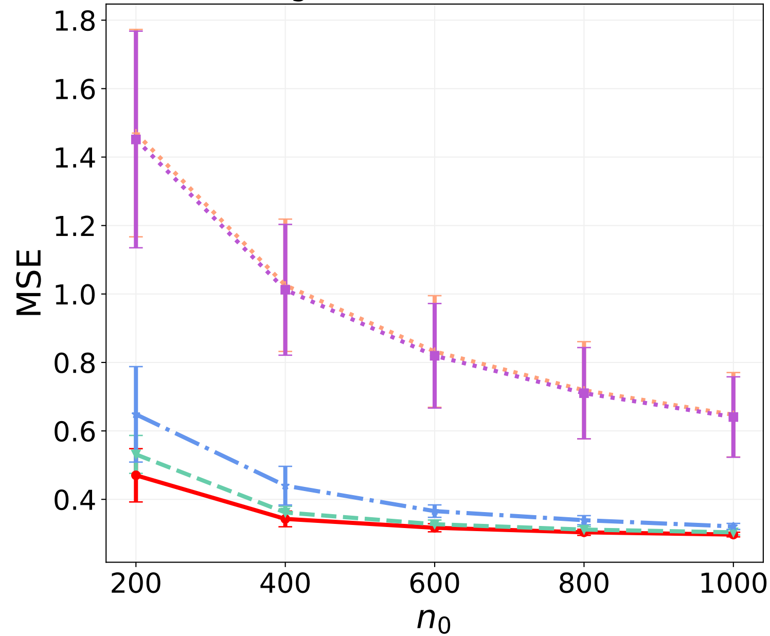
(n_s, d) = (2000, 10)
