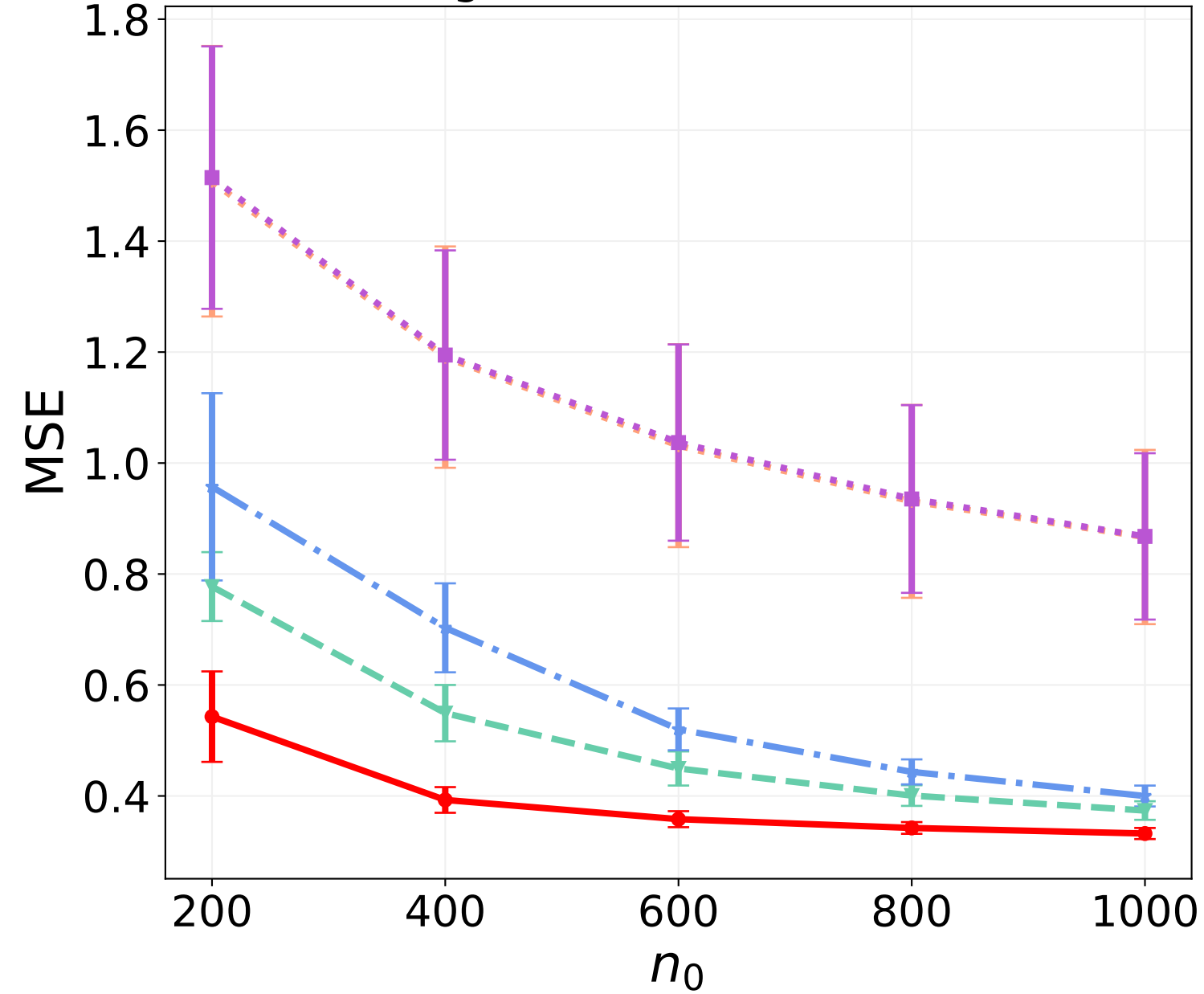
(n_s, d) = (2000, 20)
