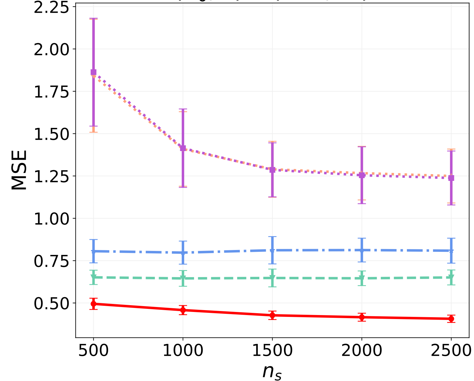
(n_0, d) = (500, 30)
