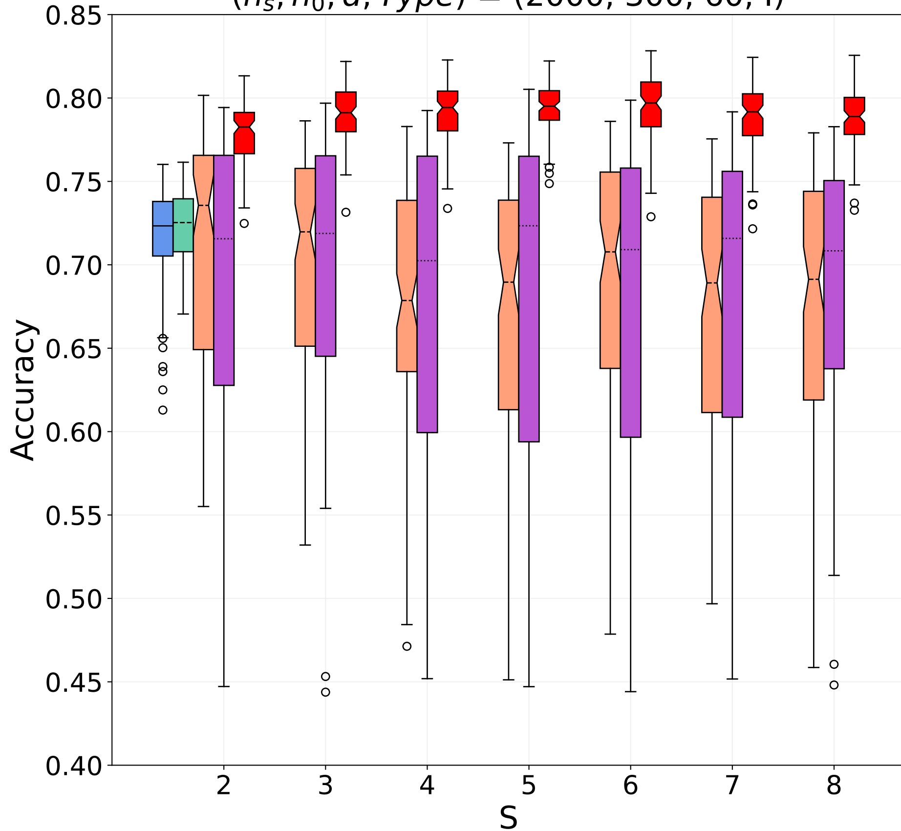
(n_s, n_0, d, \text{Type}) = (2000, 300, 60, \text{I})
