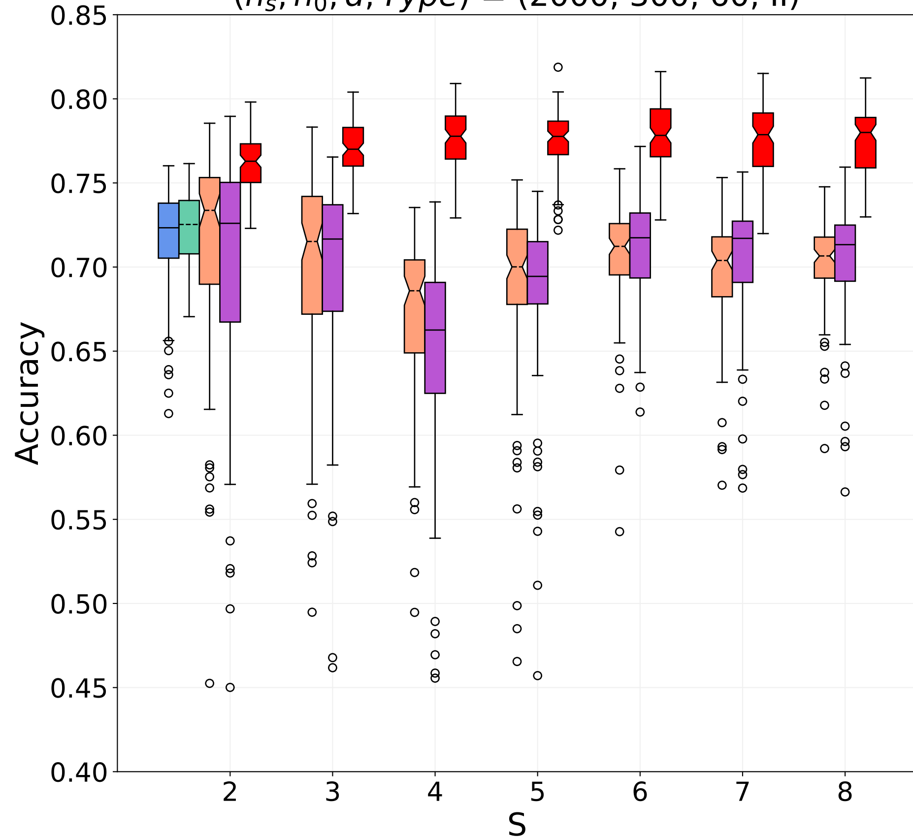
(n_s, n_0, d, \text{Type}) = (2000, 300, 60, \text{II})
