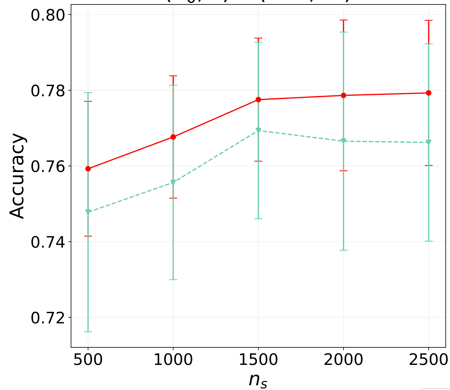
(n_0, d) = (300, 30)
