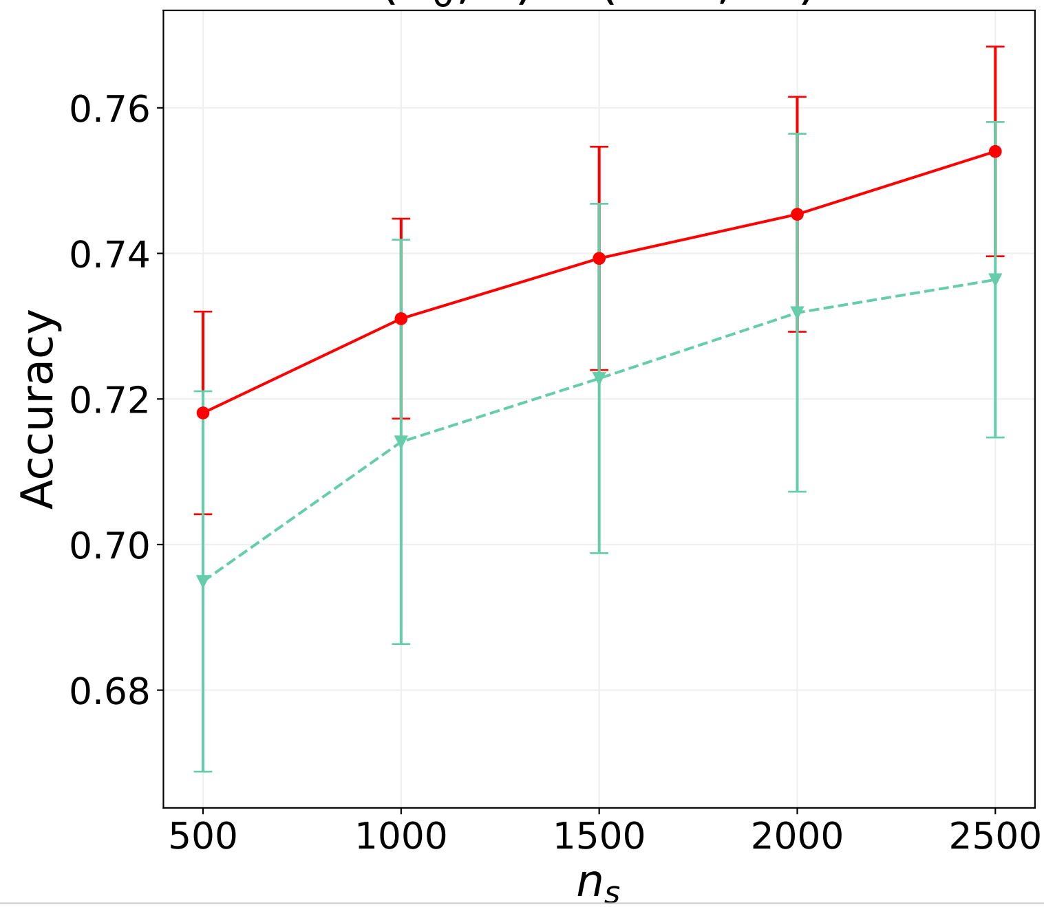
(n_0, d) = (300, 60)
