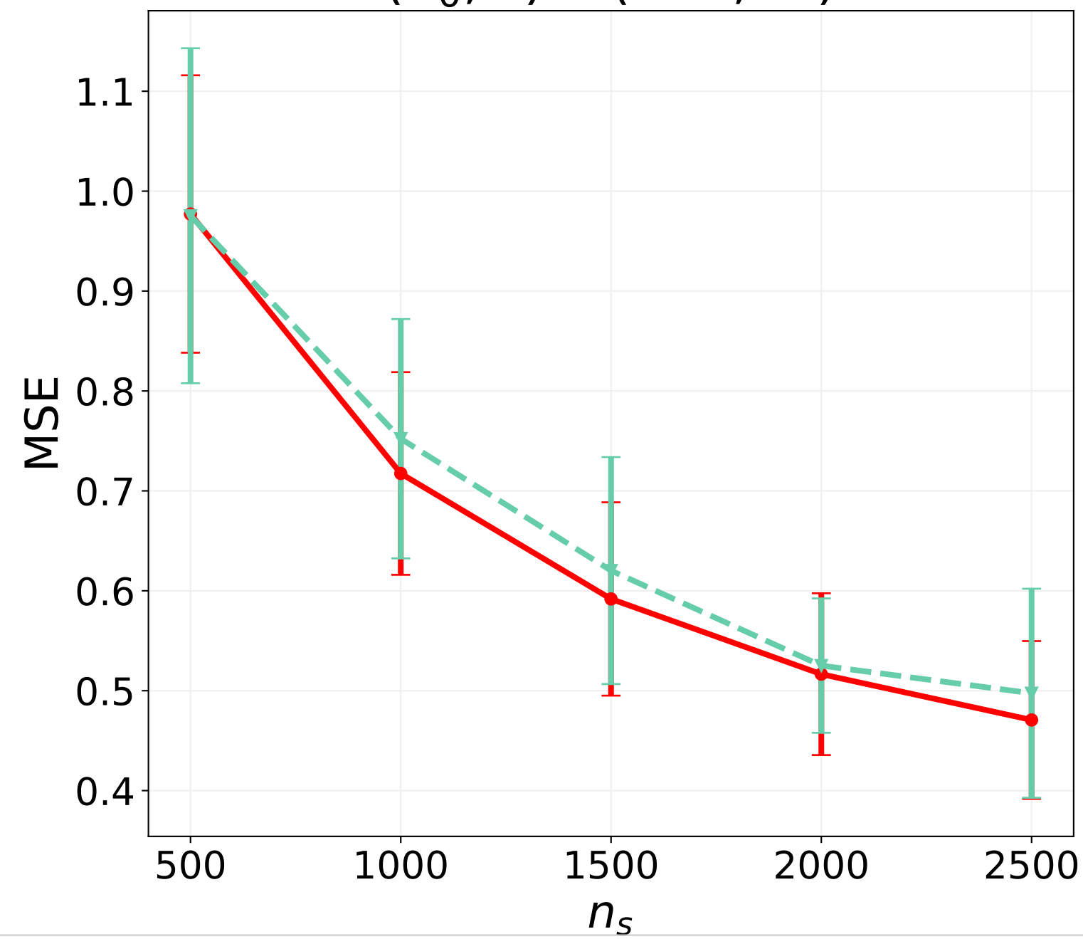
(n_0, d) = (300, 60)
