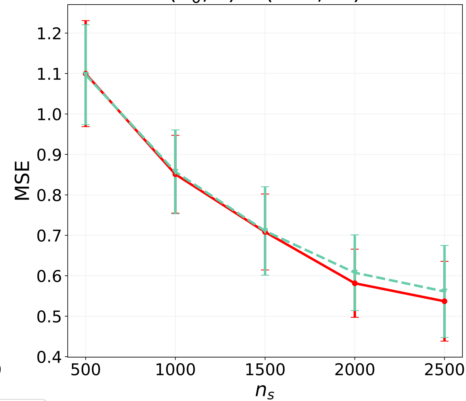
(n_0, d) = (300, 90)
