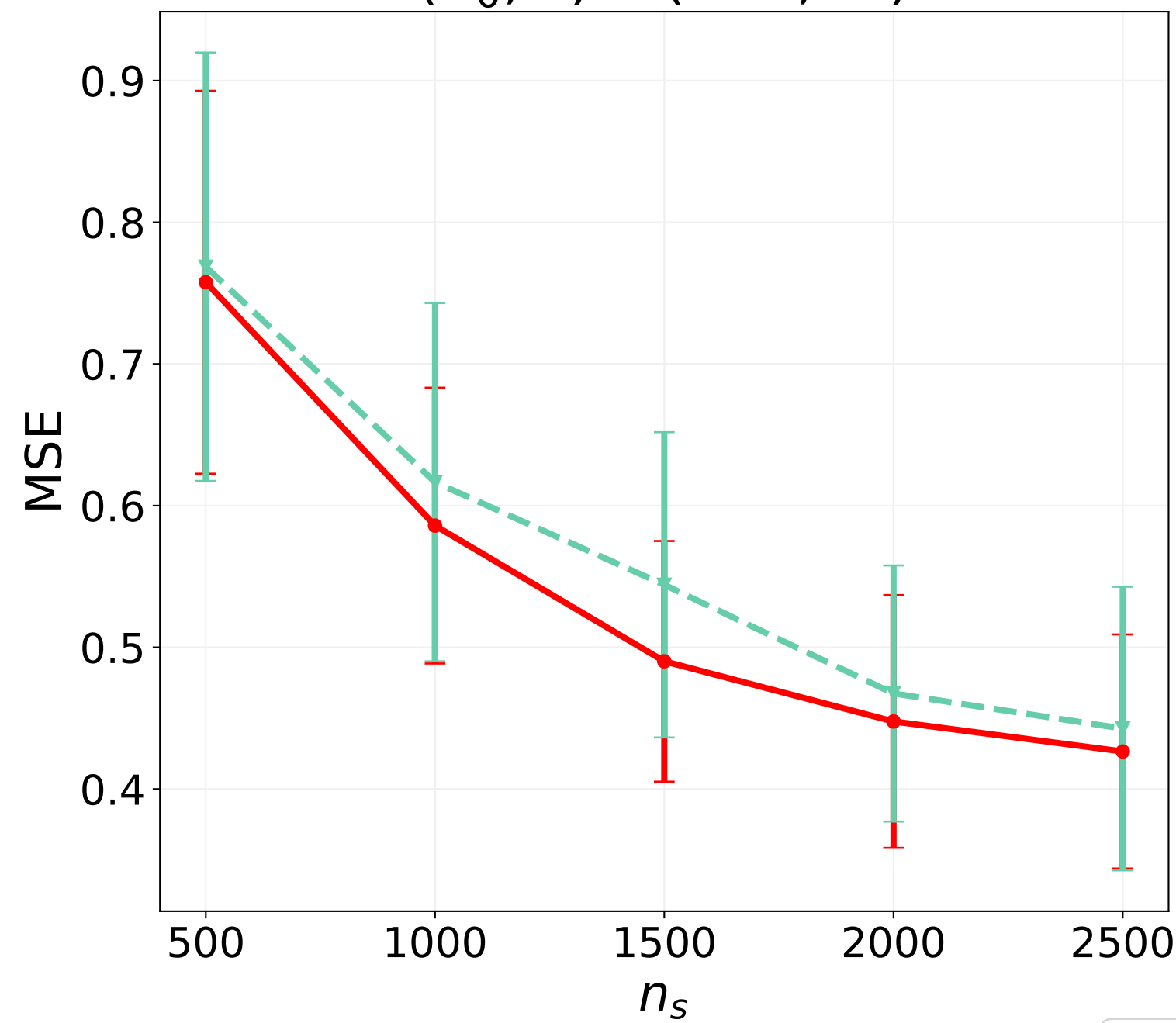
(n_0, d) = (300, 30)
