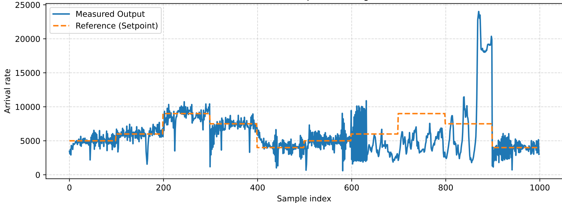
Reference vs. Measured Output (Tracking Performance)
