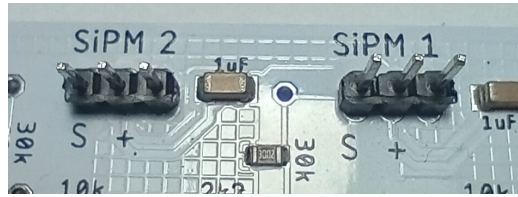
Figure 4: SiPM connection pins on the Muon Count PCB.
