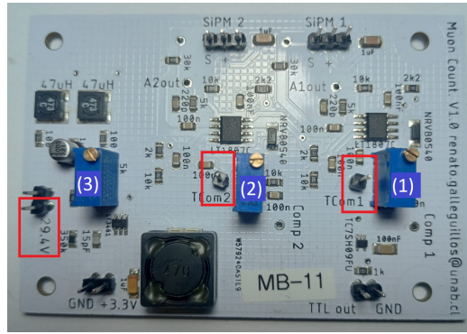
Figure 6: In blue: Muon Count PCB potentiometers. In red: Potentiometer voltage testing pins.
