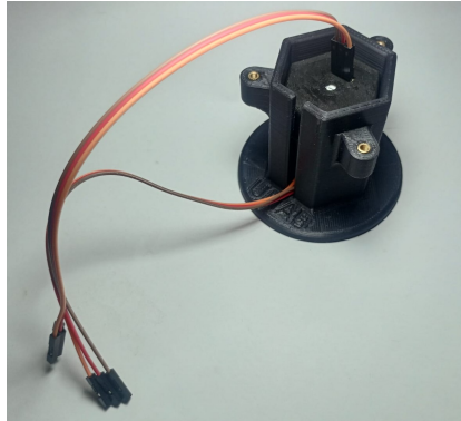
Figure 3: Assembled detector without the top cover.
