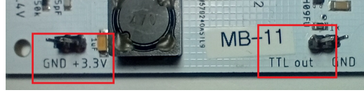
Figure 5: Arduino UNO connections pins on the Muon Count PCB.
