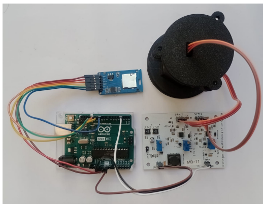
Figure 7: Complete Muon Detector setup.
