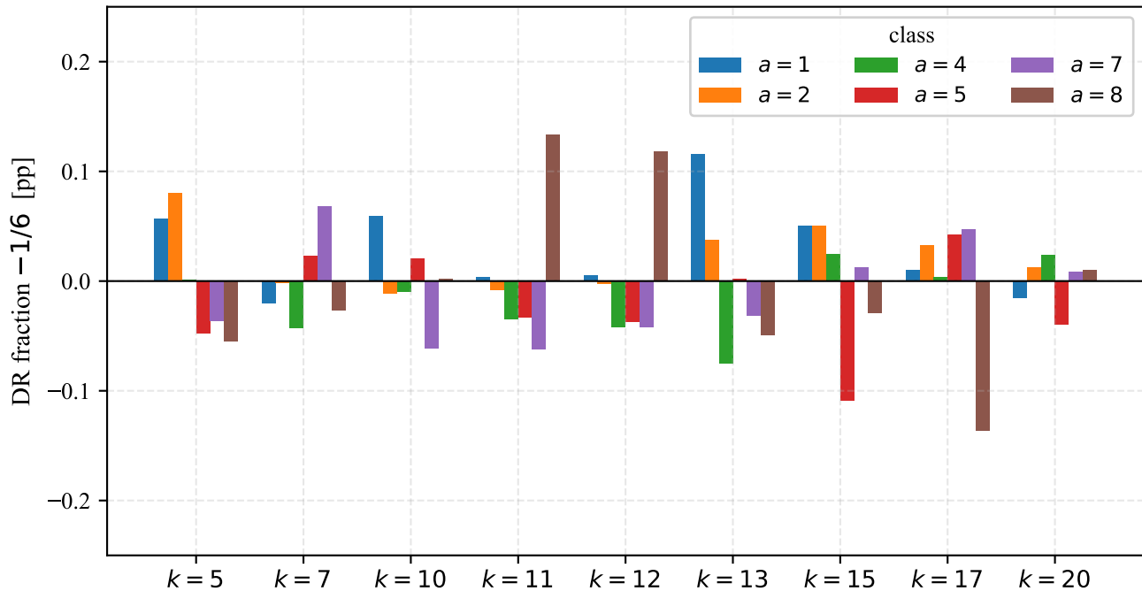
Equidistribution of DR classes for pairs (p, p + 18k)
