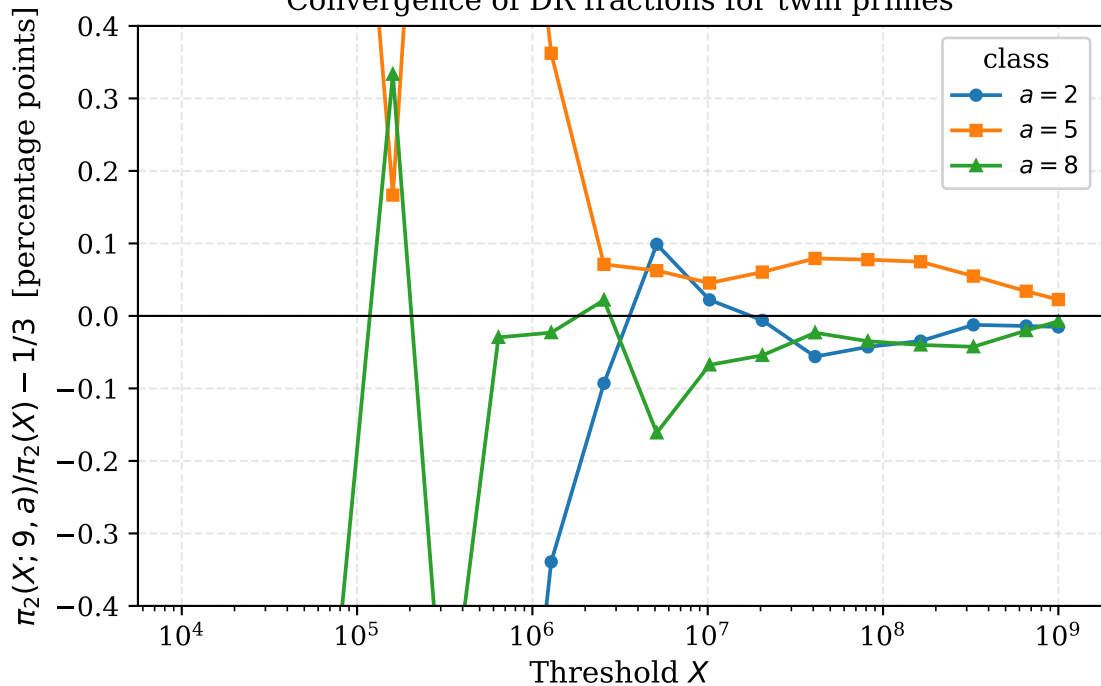
Convergence of DR fractions for twin primes
