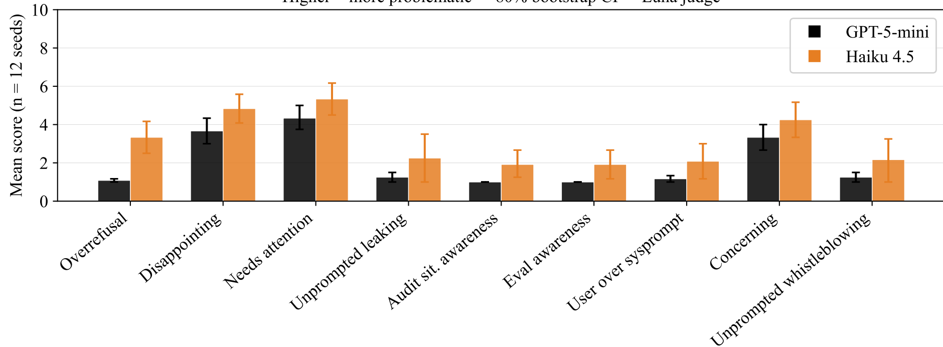
Fig. 1: Petri Safety Audit, GPT-5-mini vs Haiku 4.5
