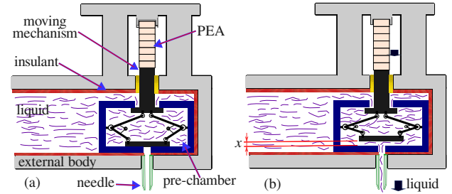
Fig. 1: The liquid drug delivery system. A voltage u applied to the PEA opens two gaps in an antagonist way: one admits liquid into the pre-chamber, the other injects it towards the needle. The delivered dose is set by the displacement x of the second gap.
