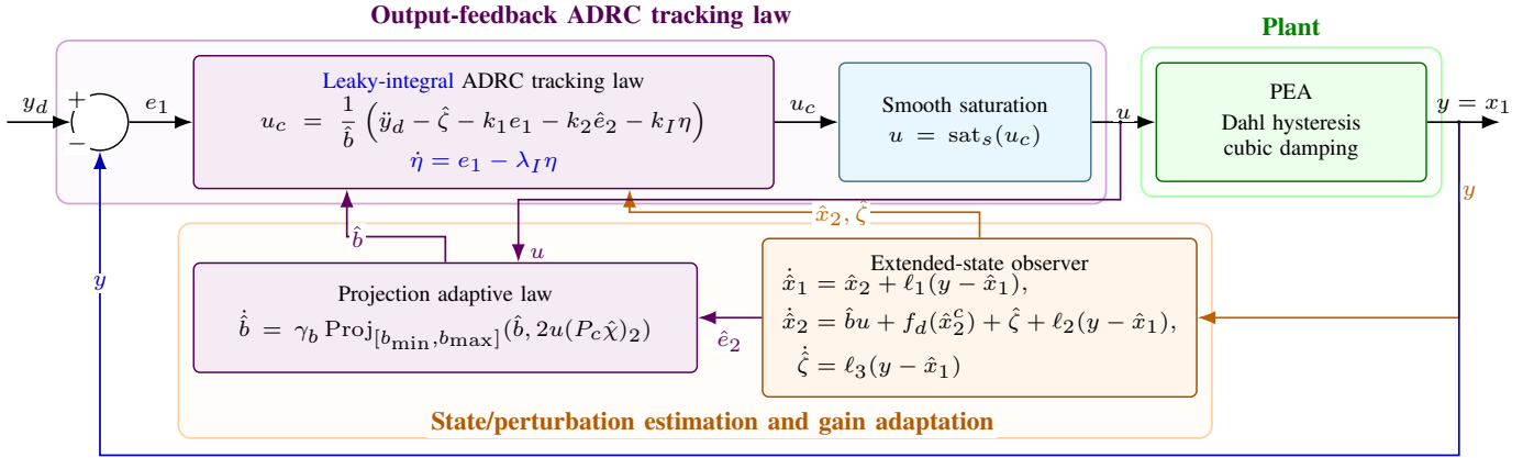
Fig. 2: Block diagram of the proposed adaptive saturated output-feedback ADRC scheme. The ESO, driven by the applied voltage u , reconstructs \hat{x}_2 and \zeta = \xi from the measured position y = x_1 ; the integral state carries a leakage \lambda_I > 0 .
