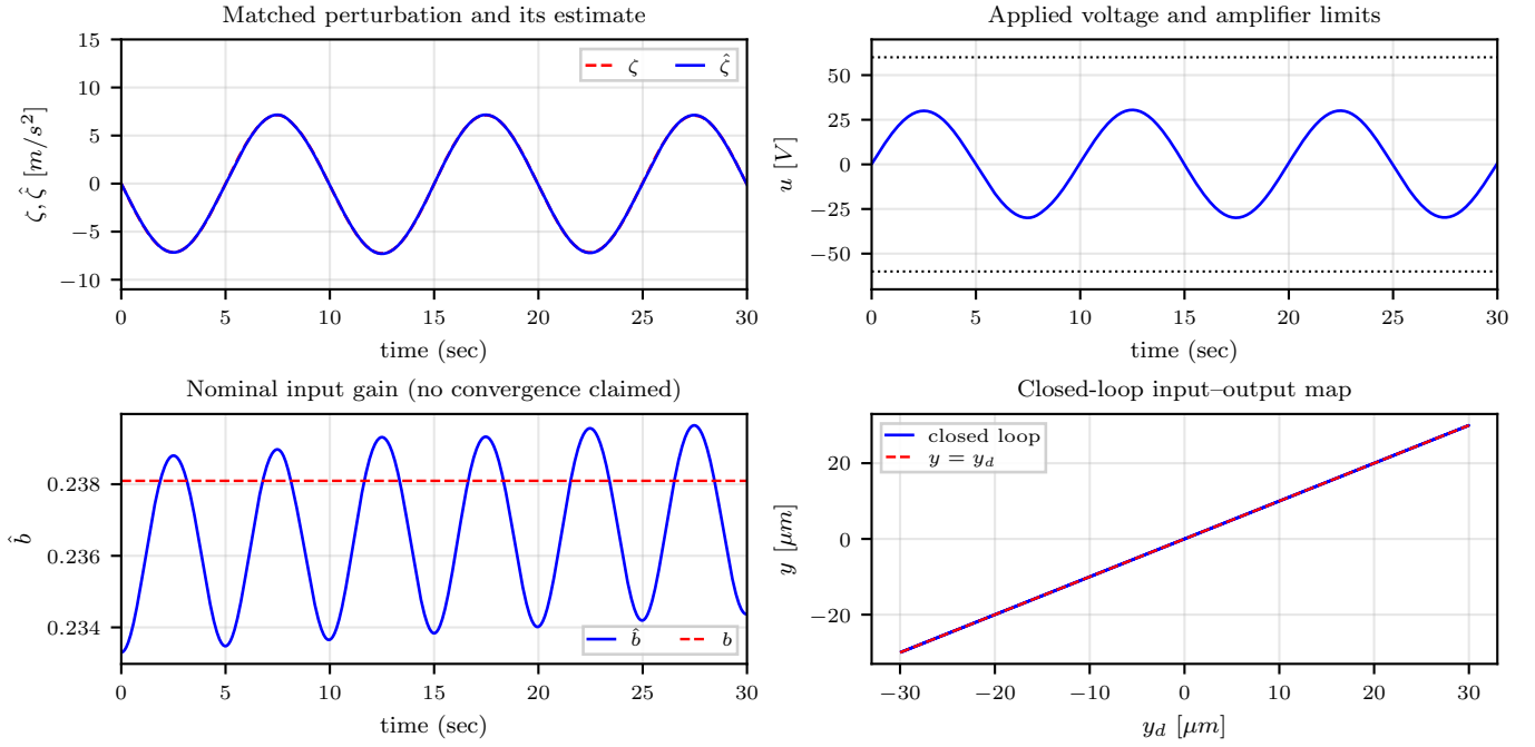
Fig. S2: Nominal run, y_d = 30 \sin(2\pi t/10) \mu\text{m} . Top left: the ESO estimate \hat{\zeta} tracks the matched plant perturbation \zeta = \xi , which collects the stiffness, hysteresis and environmental-force terms. Top right: the applied voltage stays within \pm 30.5 V, so the amplifier limits \pm u_{\max} are never reached and the saturation is inactive in this run. Bottom left: the nominal input gain \hat{b} oscillates with the reference and remains close to its initial value, slightly below the true gain b (dashed); no convergence is claimed. Bottom right: the closed-loop map (y_d, y) is indistinguishable from the ideal line y = y_d at this scale.
