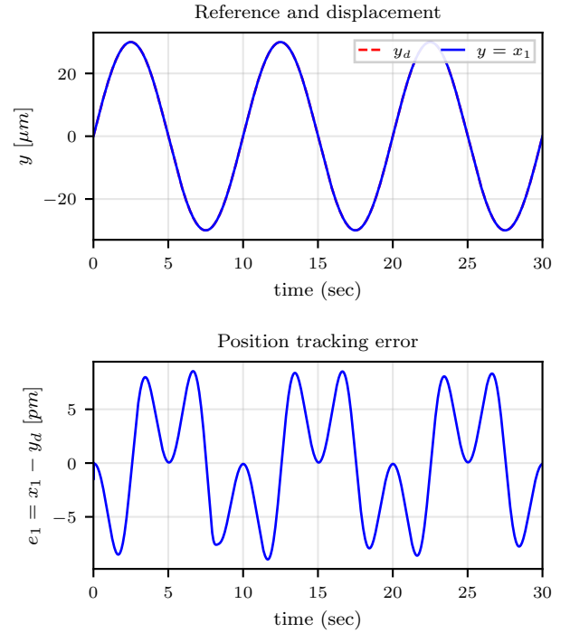
Fig. S1: Closed-loop tracking response under the adaptive saturated ADRC with the gains of Table S1. Top: reference y_d and actuator displacement y = x_1 . Bottom: position tracking error e_1 = x_1 - y_d , in picometres (1 pm = 10^{-6} \mu\text{m} ).
