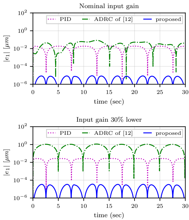
Fig. S7: Comparison with the ADRC of Flores and Rakotondrabe, ref. [12] of the letter, and with a PID with filtered derivative using the position measurement only (no observer). All three are tuned for the same closed-loop bandwidth and draw the same peak voltage. Top: nominal input gain. Bottom: the true d_p is 30% below its nominal value.
