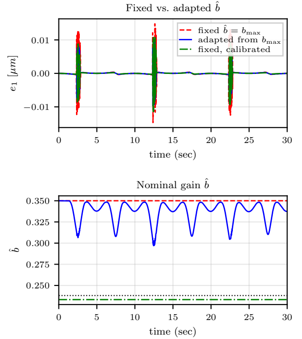
Fig. S4: Fixed versus adapted nominal input gain under active saturation. Top: position error for \hat{b} held fixed at b_{\max} , for the adaptive law started from the same value, and for the calibrated fixed value. Bottom: the corresponding \hat{b}(t) , with the true gain b dotted. In the unsaturated scenario the curves are indistinguishable.
