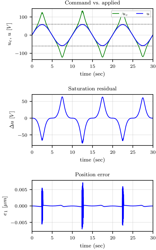
Fig. S3: Active saturation (58 \mu\text{m} reference): unsaturated command u_c and applied voltage u , saturation residual \Delta u , and position error, from top to bottom. The actuator is saturated during 42% of the run.
