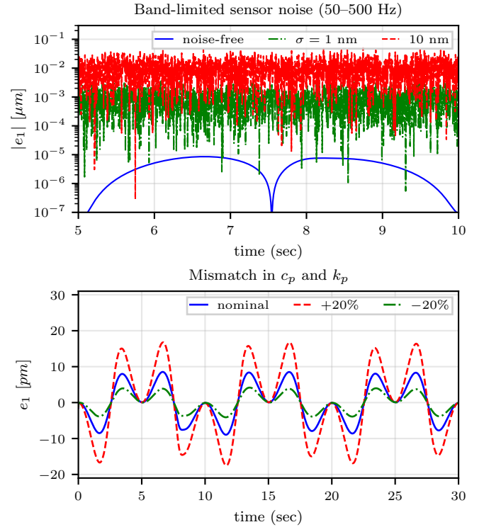
Fig. S6: Robustness. Top: band-limited (50–500 Hz) sensor noise, 10 s horizon. Bottom: \pm 20\% mismatch in c_p and k_p , 30 s horizon. Same solver and tolerances as the remaining runs.
