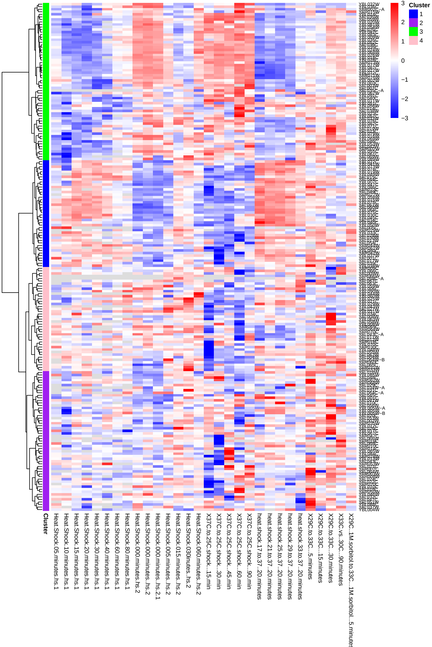
Yeast Cluster Heatmap
