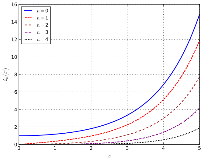
Figure 3.9: Plot of the function i_n(x) versus x for n=0, 1, 2, 3, 4 . The curves are ordered by their values at x=5 , with n=0 having the highest value and n=4 having the lowest.
