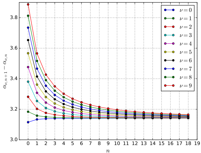
Figure 6.2: Difference between consecutive values of the function \mathcal{I}(\cdot) for different values of \nu .
