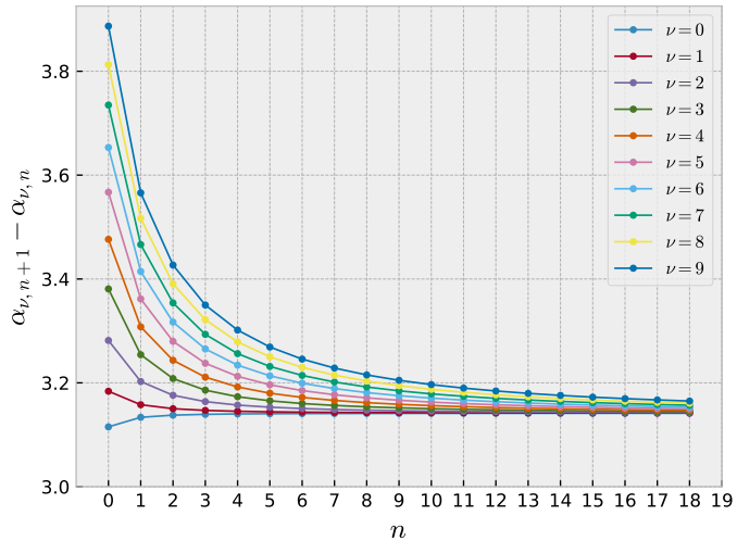
Figure 6.2: Difference between consecutive values of the function \mathcal{I}(\cdot) for different values of \nu .
