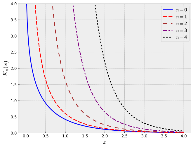
Figure 3.6: Plot of the function K_n(x) versus x for n = 0, 1, 2, 3, 4 . The curves are shifted to the right as n increases.
