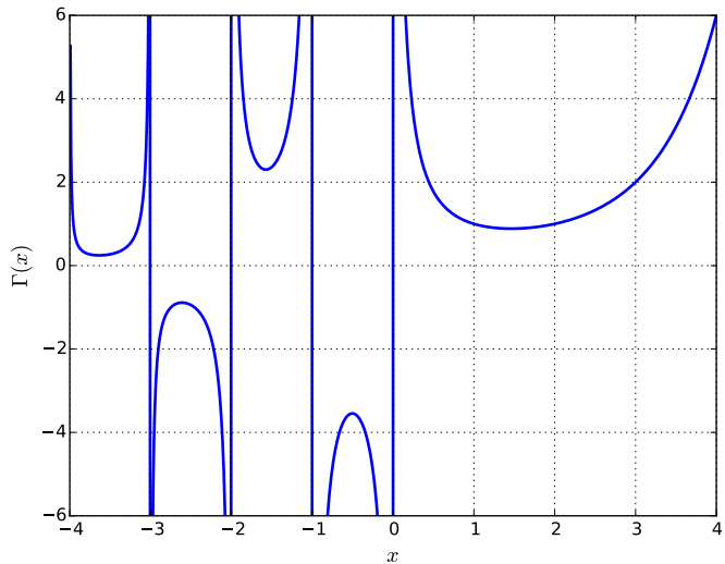
Fig. 1.1. Gamma function \Gamma(x) for x \in (-4, 4) . The function is defined for all real numbers except at the non-positive integers.
