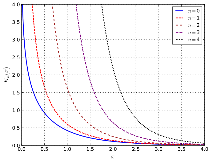
Figure 3.6: Plot of the function K_n(x) versus x for n = 0, 1, 2, 3, 4 . The curves are shifted to the right as n increases.
