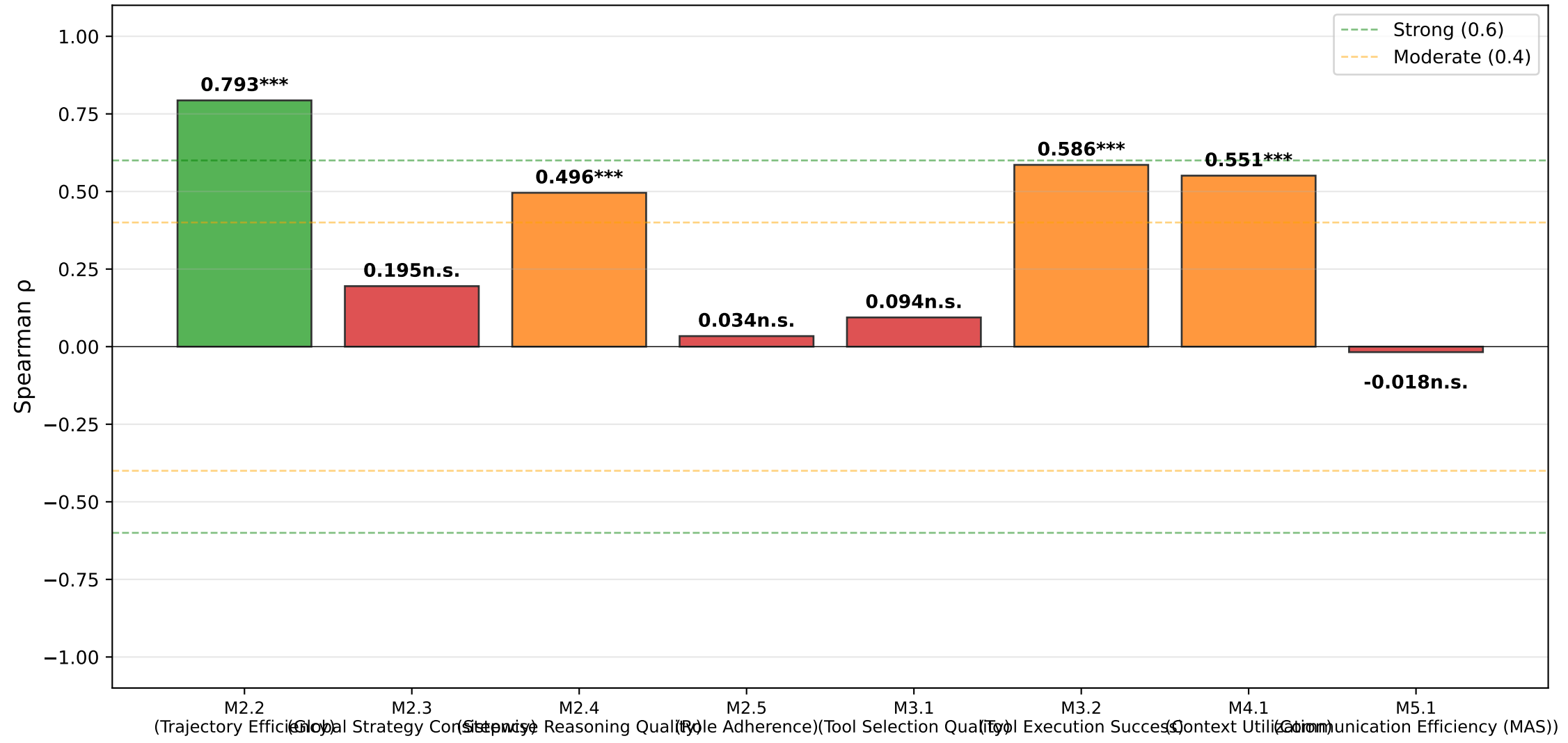
Spearman Correlation: Auto Scores vs. Human Expert Scores
