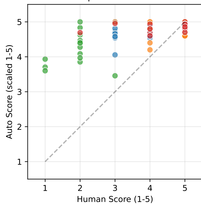
M4.1: Context Utilization \rho=0.520 ***
