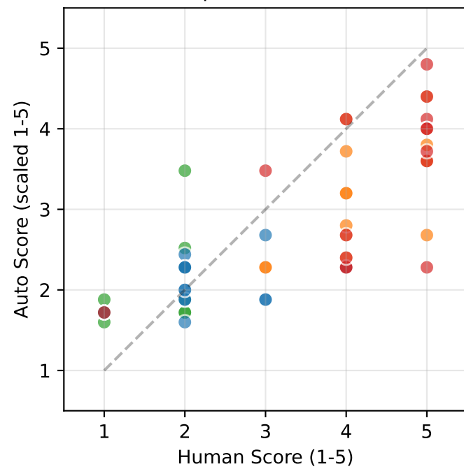
M2.5: Role Adherence \rho=0.336 **
