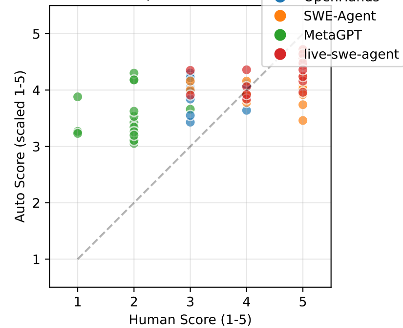
M3.2: Tool Execution Success \rho=0.446 ***
