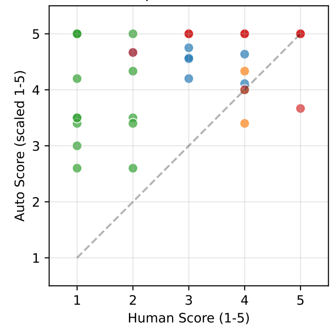
M3.2: Tool Execution Success \rho=0.446 ***
