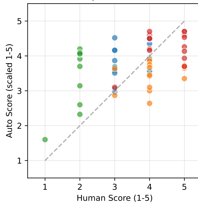
M5.1: Communication Efficiency (MAS) \rho=0.097 n.s.
