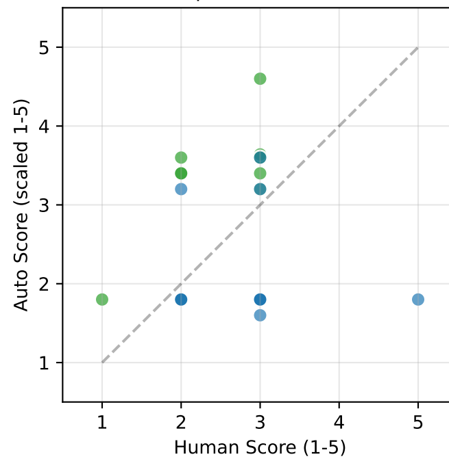
M3.1: Tool Selection Quality \rho=0.268 *
