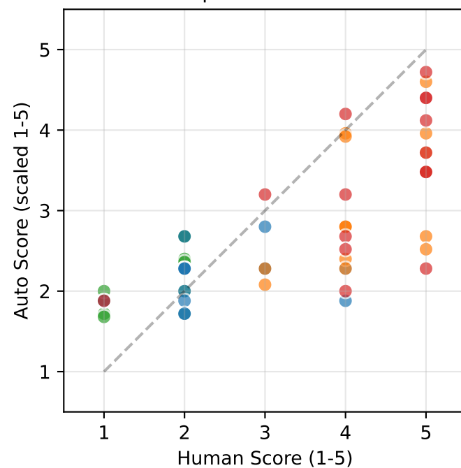
M2.5: Role Adherence \rho=0.264 *
