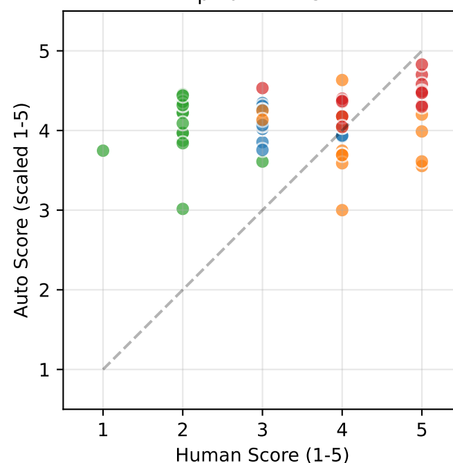
M5.1: Communication Efficiency (MAS) \rho=0.685 **
