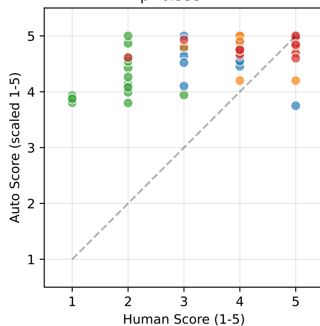
M4.1: Context Utilization \rho=0.533 ***
