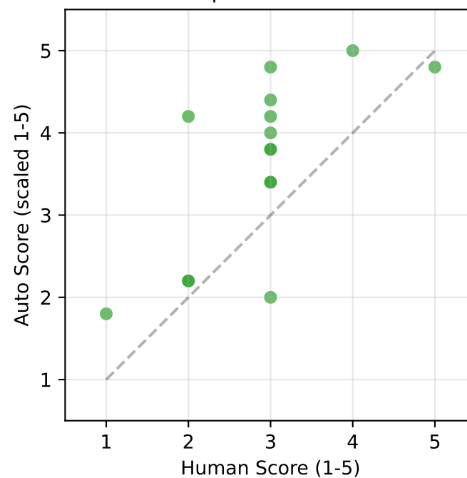
M3.1: Tool Selection Quality \rho=0.177 n.s.
