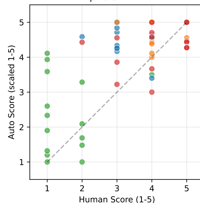
M3.2: Tool Execution Success \rho=0.627 ***
