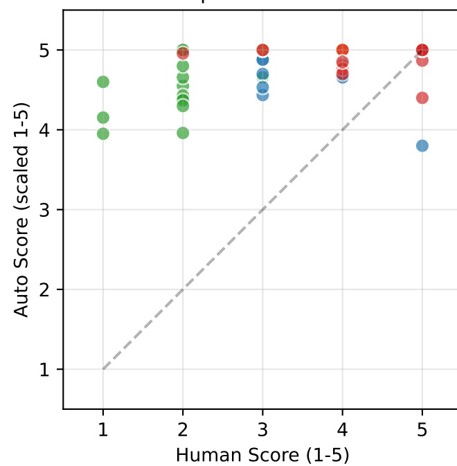
M4.1: Context Utilization \rho=0.555 ***
