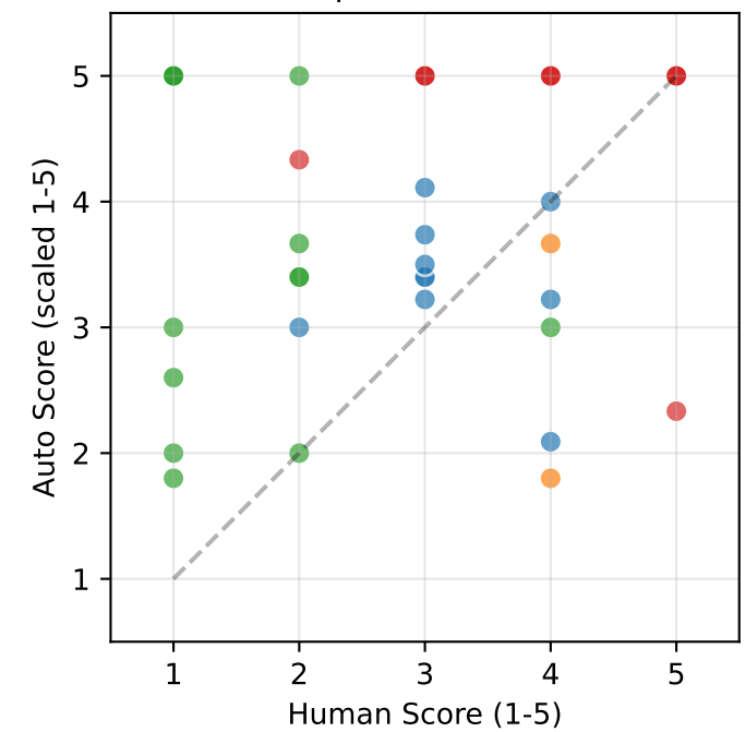
M3.2: Tool Execution Success \rho=0.342 **
