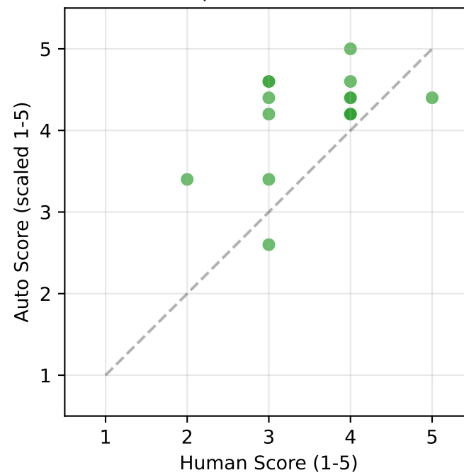
M3.1: Tool Selection Quality \rho=0.198 n.s.
