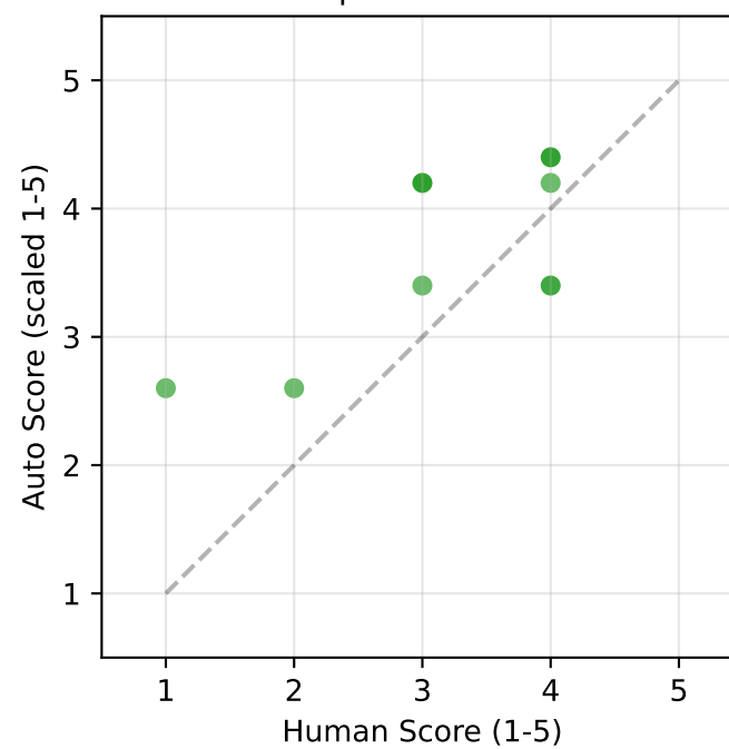
M5.1: Communication Efficiency (MAS) \rho=0.540 *
