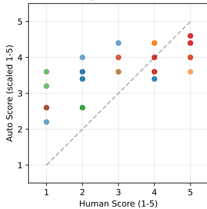
M2.5: Role Adherence \rho=0.327 *
