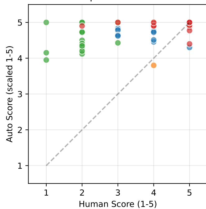
M4.1: Context Utilization \rho=0.479 ***
