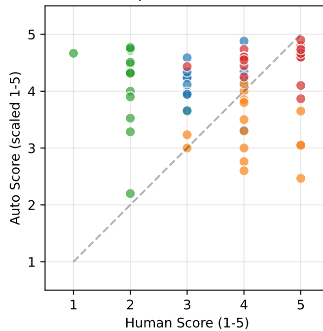
M5.1: Communication Efficiency (MAS) \rho=0.543 *
