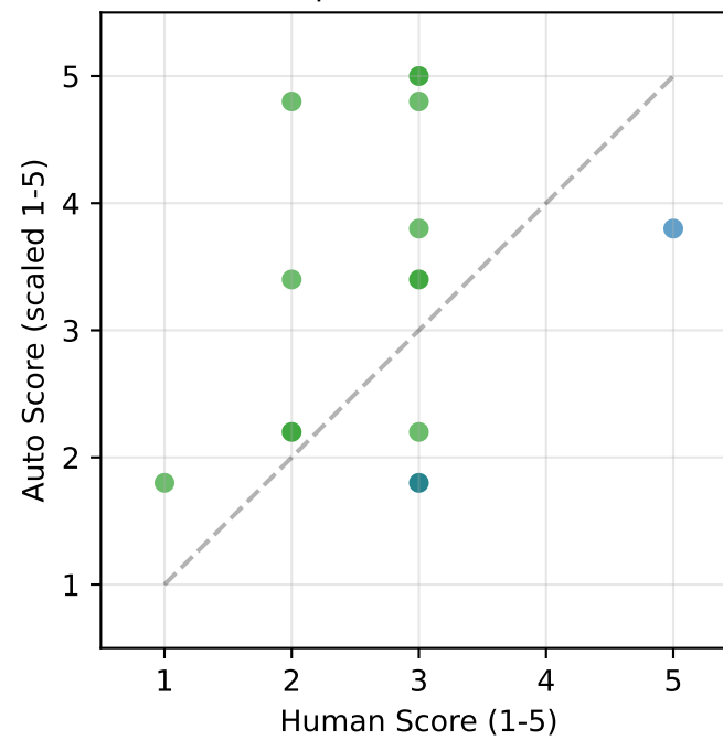
M3.1: Tool Selection Quality \rho=-0.025 n.s.
