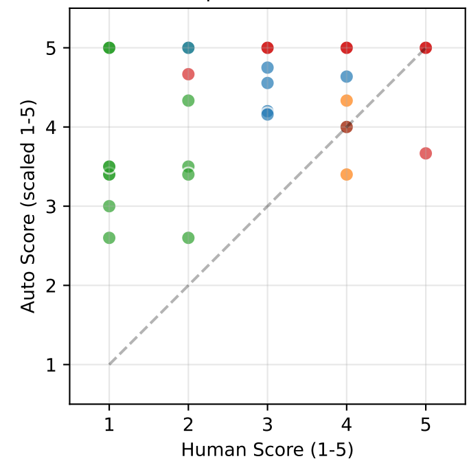
M3.2: Tool Execution Success \rho=0.455 ***
