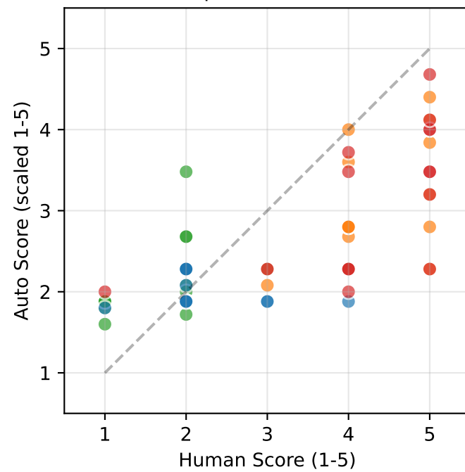
M2.5: Role Adherence \rho=0.273 *
