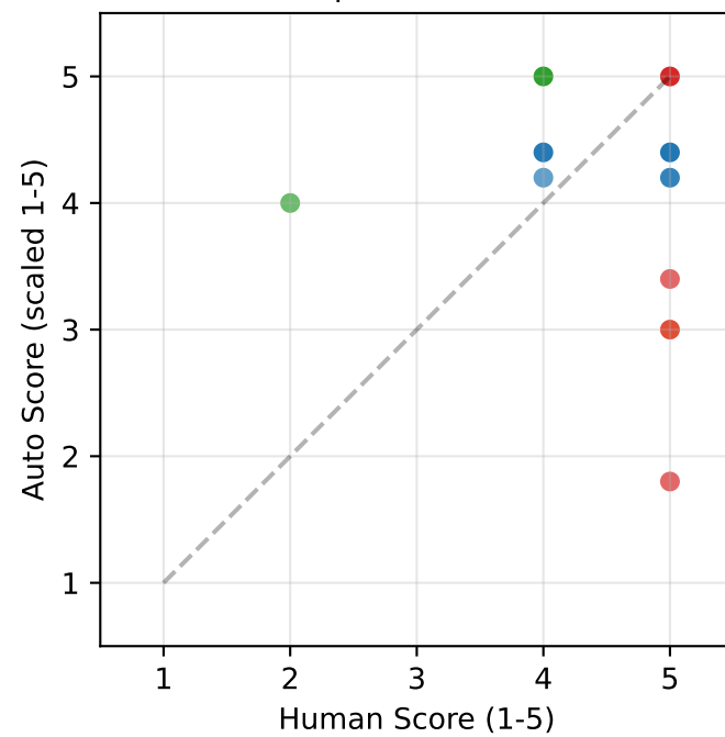
M4.1: Context Utilization \rho=0.569 ***
