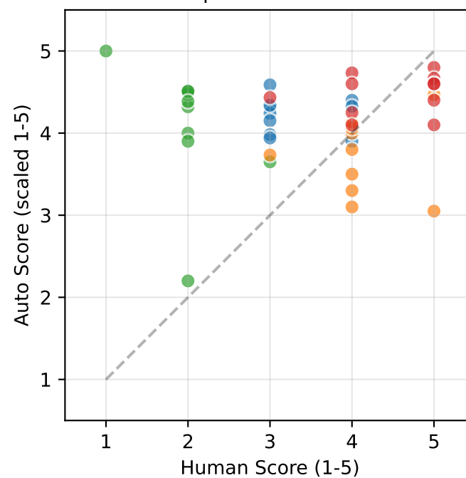
M5.1: Communication Efficiency (MAS) \rho=0.038 n.s.
