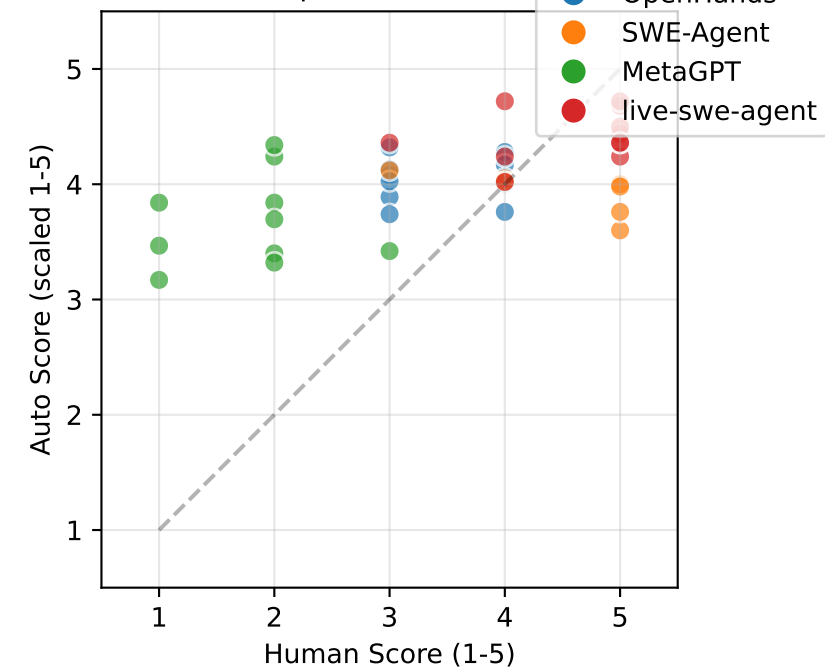
M3.2: Tool Execution Success \rho=0.326 *
