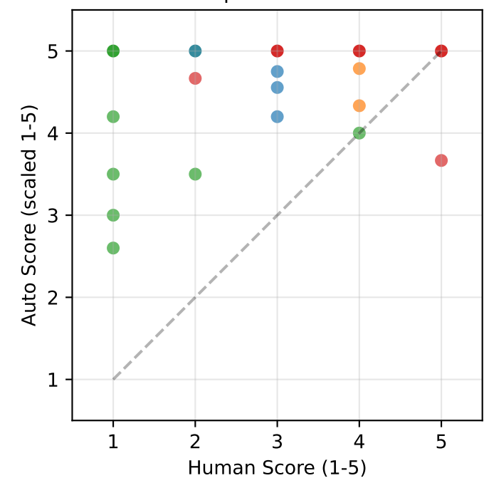
M3.2: Tool Execution Success \rho=0.326 *
