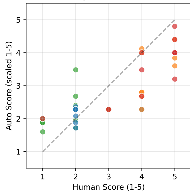
M2.5: Role Adherence \rho=0.352 *
