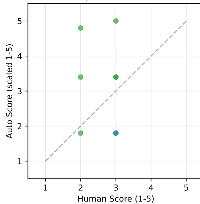
M3.1: Tool Selection Quality \rho=0.073 n.s.
