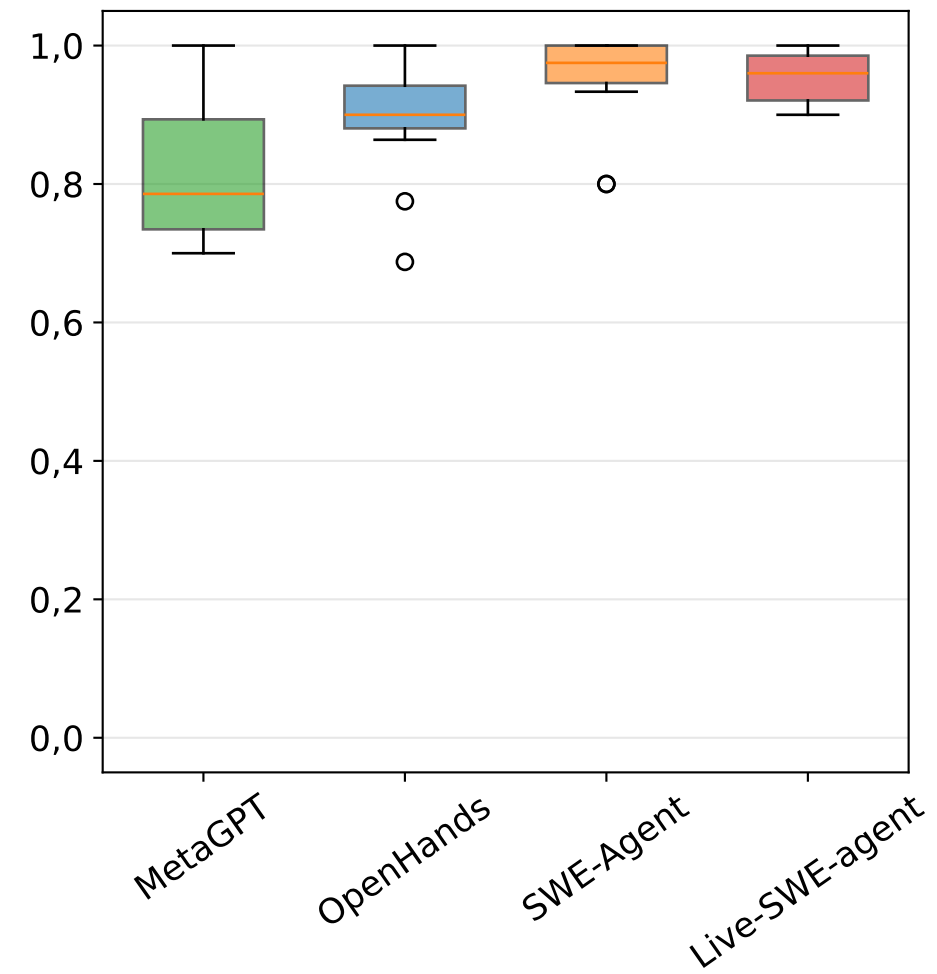
M4.1 Context Utilization
