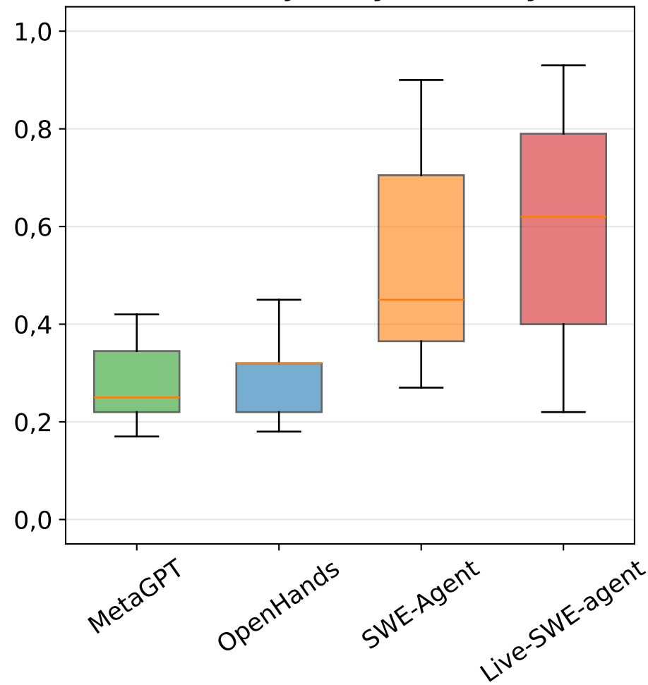
M3.1 Tool Selection Quality
