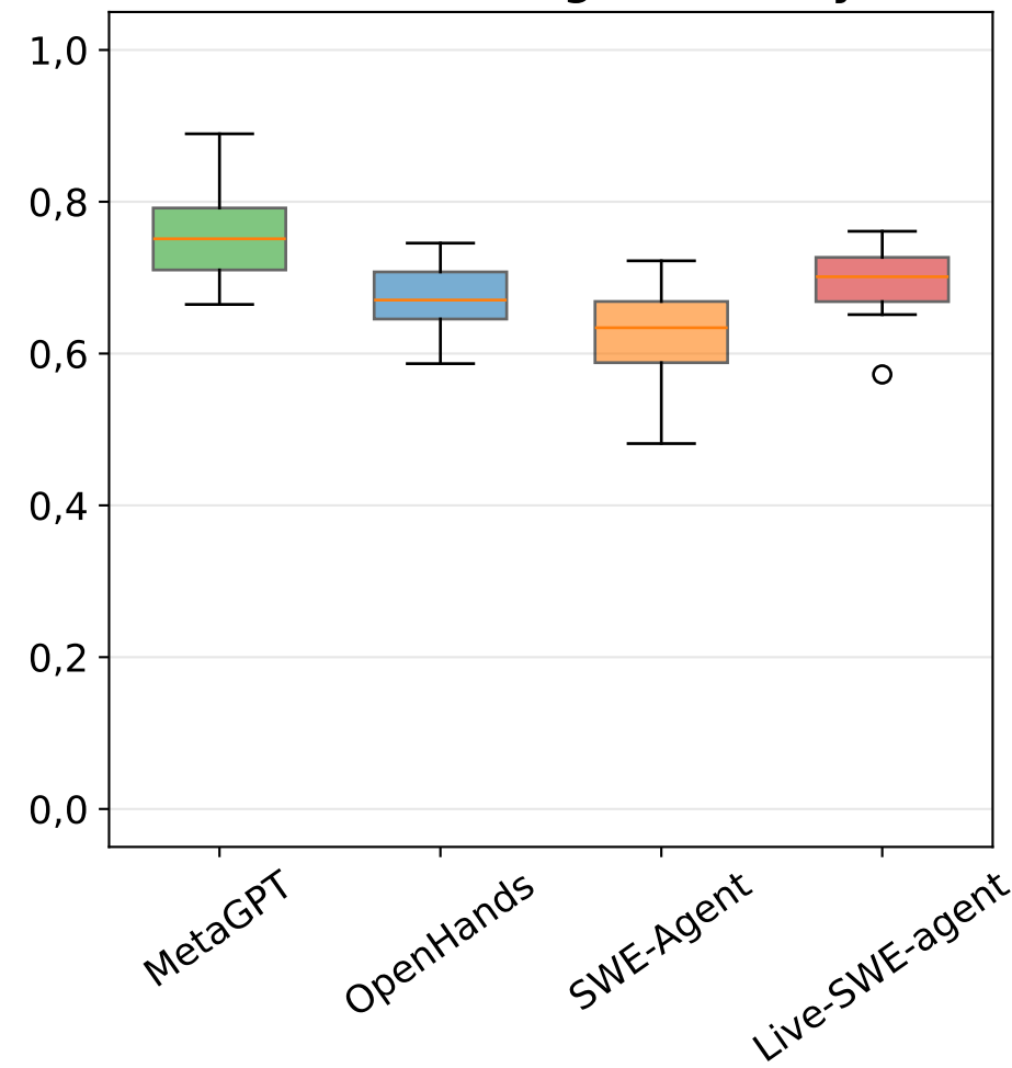
M3.3 Tool Usage Efficiency
