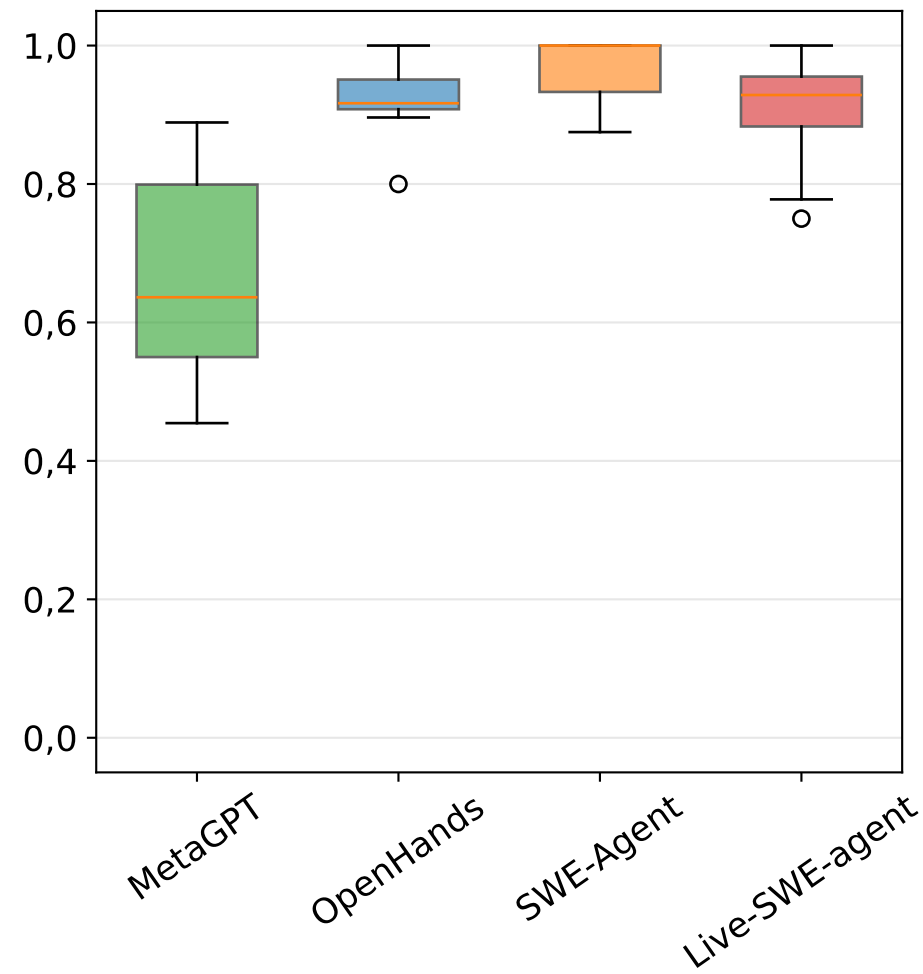
M3.2 Tool Execution Success
