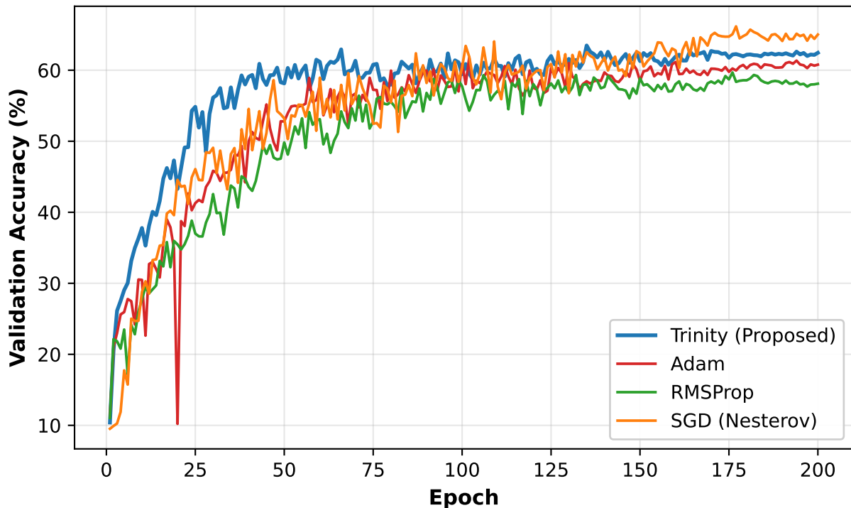
Exp 1: Wide-ResNet-101-2 — Validation Accuracy
