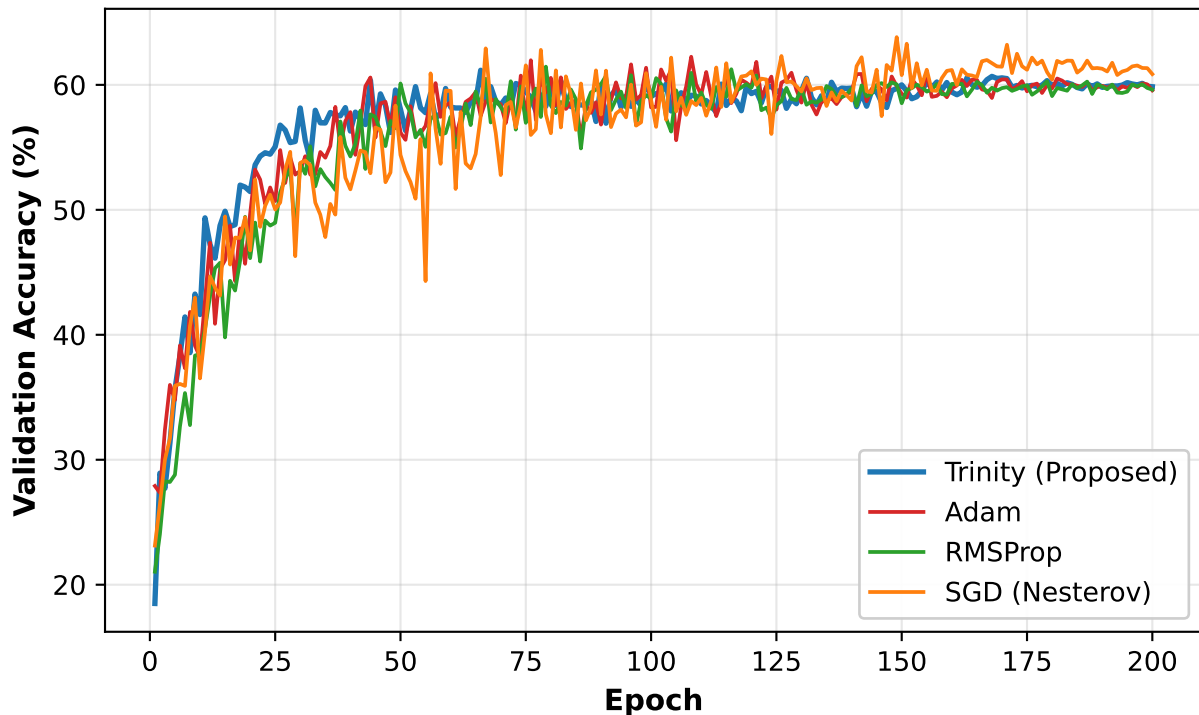
Exp 3: ResNet-18 — Validation Accuracy
