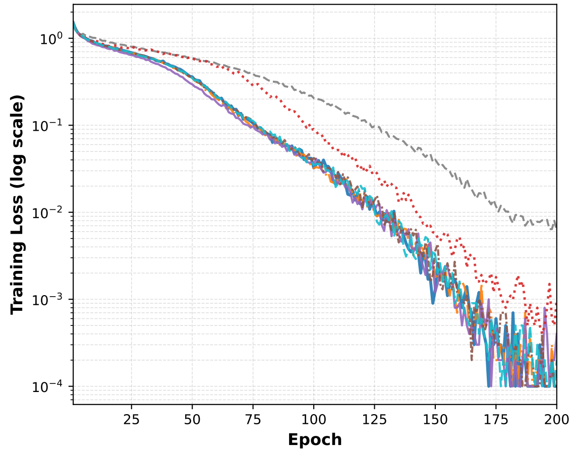
Vision Transformer (Exp. 2)
