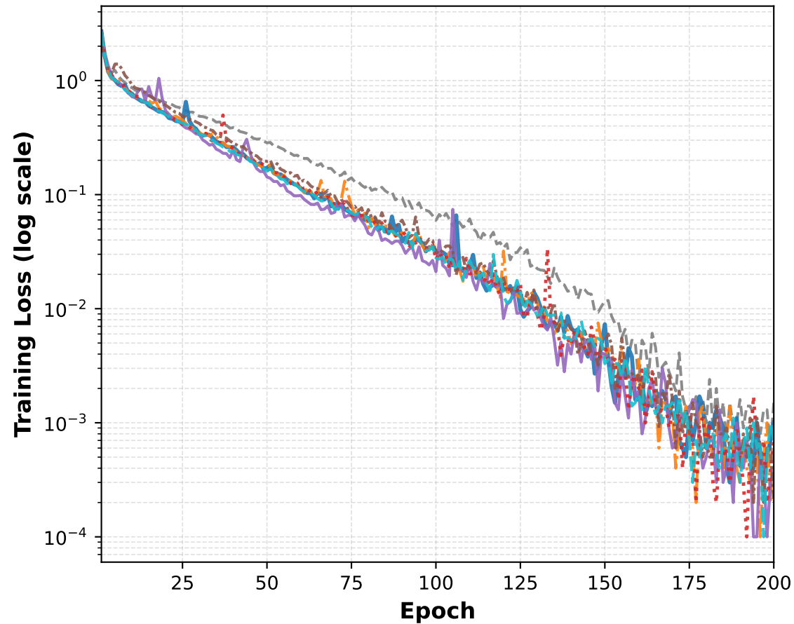
Wide-ResNet-101-2 (Exp. 1)
