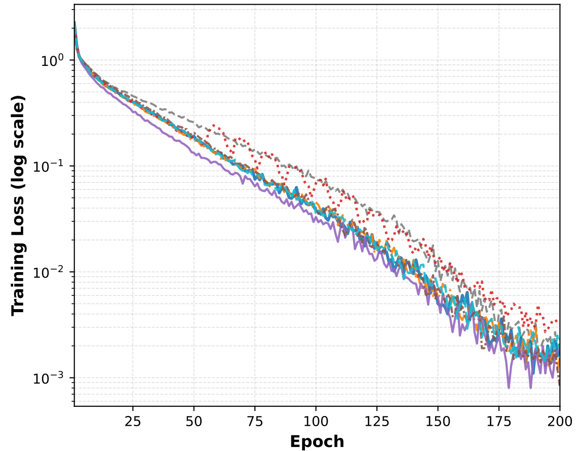
ResNet-18 (Exp. 3)
