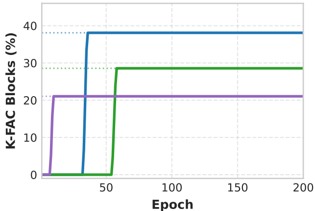
(a) K-FAC Allocation (%)
