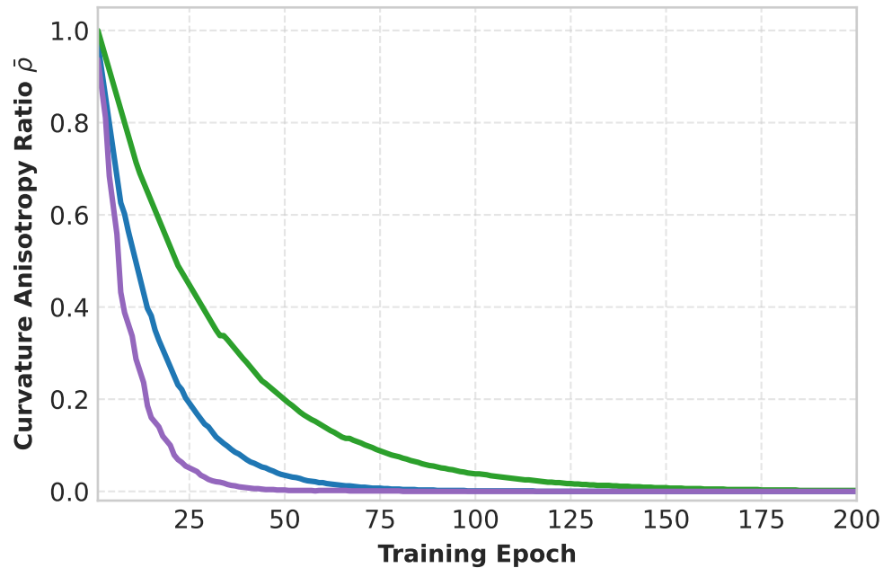
(b) Spectral Anisotropy Evolution ( \bar{\rho} )
