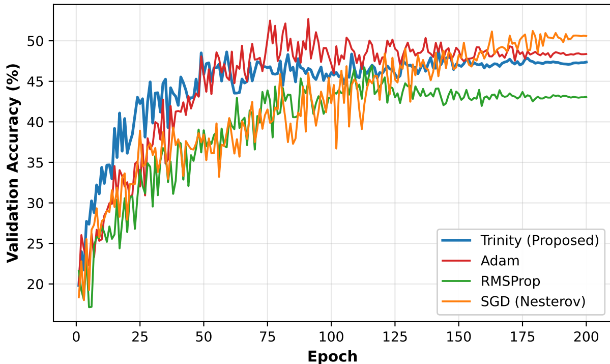
Exp 2: Vision Transformer — Validation Accuracy
