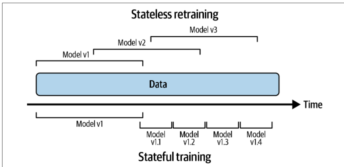
Figure 9-2. Stateless retraining versus stateful training
