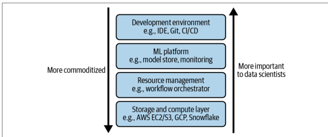
Figure 10-2. Different layers of infrastructure for ML
