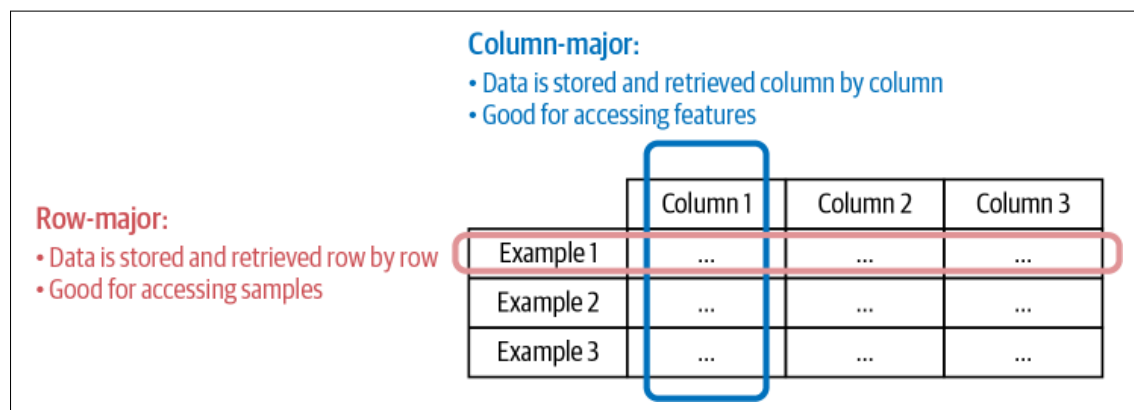
Figure 3-1. Row-major versus column-major formats
