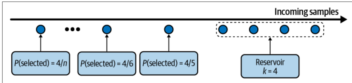
Figure 4-2. A visualization of how reservoir sampling works
