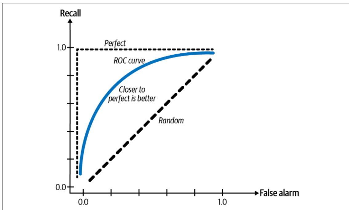
Figure 4-9. ROC curve
