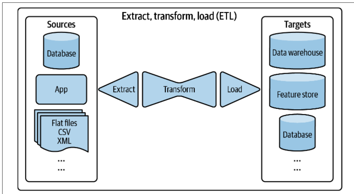
Figure 3-7. An overview of the ETL process
