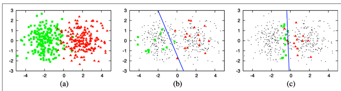
Figure 4-7. How uncertainty-based active learning works. (a) A toy dataset of 400 instances, evenly sampled from two class Gaussians. (b) A model trained on 30 samples randomly labeled gives an accuracy of 70%. (c) A model trained on 30 samples chosen by active learning gives an accuracy of 90%. Source: Burr Settles 22
