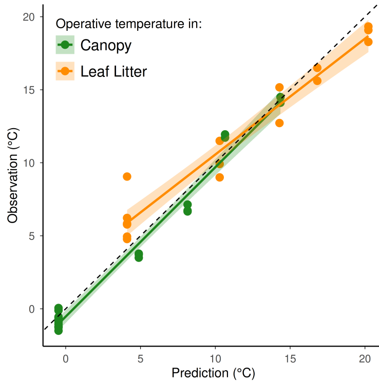
Figure S8. Validation of the minimum operative temperatures estimated by our biophysical models against those recorded by operative temperature models (OTMs) at five locations across the latitudinal range of the American green anole ( Anolis carolinensis ). Each point shows the mean daily minimum temperature recorded by one OTM between 11 and 19 January (observation) against the minimum operative temperature predicted for its location and microhabitat (prediction; canopy at 1.8 m and leaf litter at 8 cm, the midpoint of the depths at which litter OTMs were deployed). Point colors indicate the microhabitat, and solid lines and shaded areas the best-fit line and standard error of a linear model for each microhabitat. The dashed black line indicates the 1:1 relationship. Predictions closely matched observations in the canopy (bias = 0.45 °C; RMSE = 0.88 °C; n = 22 OTMs) and in the leaf litter (bias = -0.41 °C; RMSE = 1.76 °C; n = 17 OTMs; Table S10).
