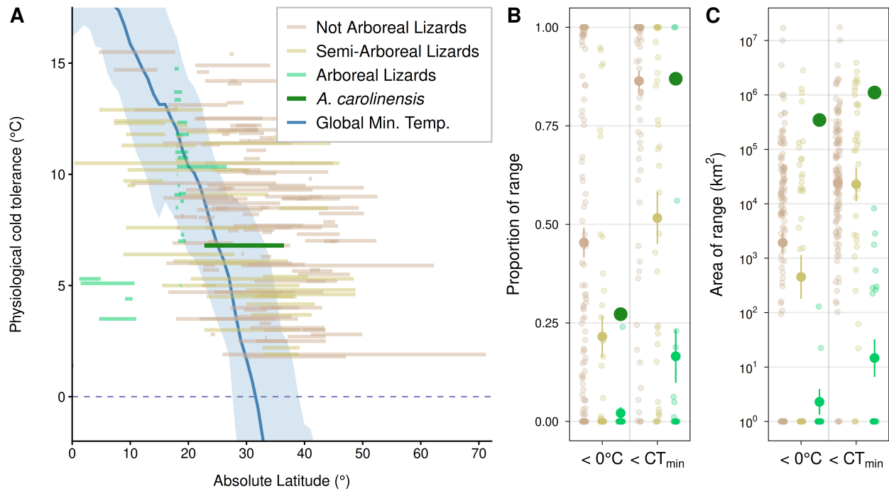
Figure S3. The American green anole ( Anolis carolinensis ) is an exceptional case of mismatch between realized and fundamental cold thermal limits among arboreal lizards. (A) The latitudinal range of each of the 180 lizard species in our dataset, placed at the height of its critical thermal minimum ( CT_{min} ) and colored by substrate use (exclusively arboreal, semi-arboreal or other), compared with the global mean ( \pm SD) minimum temperature of the coldest month (BIO6; blue line and area) at each latitude. The range of the green anole (dark green) extends into latitudes where BIO6 is well below its CT_{min} (6.8 ^{\circ}C , the lowest population-average CT_{min} across its range). (B, C) Proportion (B) and area (C, log scale) of each species' range below its CT_{min} and below 0 ^{\circ}C . Points with error bars show the mean ( \pm SE) of each substrate group, and the large dark green point the green anole. Only a few other exclusively arboreal species have ranges that extend below their CT_{min} (four Chamaeleo and four Anolis species), and only two below 0 ^{\circ}C ( Chamaeleo hoehnelii and C. schubotzi ); in all cases, the area affected is orders of magnitude smaller than for the green anole. Substrate use follows SquamBase, except for Liolaemus tenuis , which we classified as semi-arboreal because it adopts a saxicolous/terrestrial strategy in many parts of its range.
