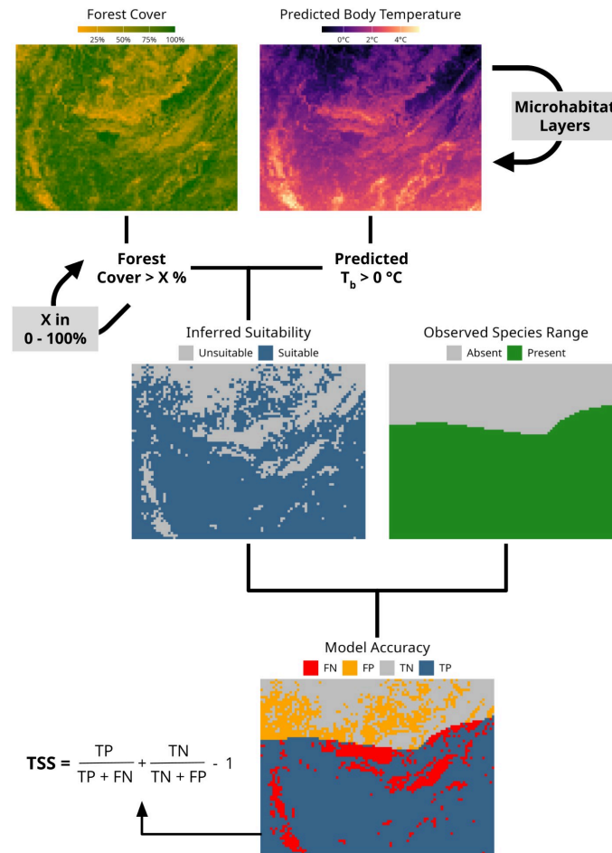
Figure S9. Diagram of our mechanistic envelope modeling approach. We start by obtaining spatially explicit data on a set of ecological variables of interest, in our case forest cover and environmental temperature, and use both layers to derive new layers of predicted lizard body temperatures across a range of microhabitats using biophysical models (Supporting Text). We then select a given microhabitat layer and set a percentage of forest cover as a threshold. Combining these two layers, we create an inferred suitability layer, assigning as suitable all spatial cells where forest cover is greater than the selected threshold and where the predicted minimum annual body temperature of the lizard ( T_b ) is greater than 0\text{ }^{\circ}\text{C} . Next, we compare the inferred suitability layer with the observed species range cell by cell, classifying each cell as a false negative (FN; red) if we infer it unsuitable but it falls within the species range, a false positive (FP; orange) if we infer it suitable but it falls outside the range, a true negative (TN; gray) if we infer it unsuitable and it falls outside the range, or a true positive (TP; blue) if we infer it suitable and it falls within the range. Lastly, we calculate the true skill statistic (TSS) of each combination of microhabitat and forest cover threshold. We repeat this process for every microhabitat layer and every forest cover threshold (0 to 100% at 5% intervals) within a given area, and identify the combination that maximizes TSS.
