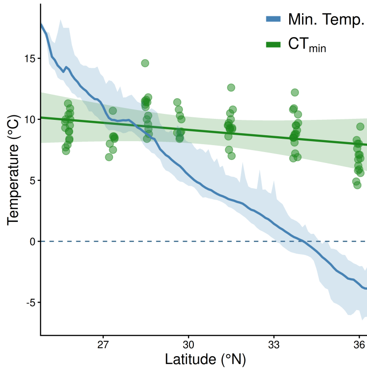
Figure S2. Latitudinal variation in the minimum temperature of the coldest month (BIO6, shown as Min. Temp.; blue) and the critical thermal minimum (CT min ; green) of American green anoles ( Anolis carolinensis ). For BIO6, the solid line and shaded area show the mean and range (minimum to maximum) of values within each 0.1° latitude band of a bounding box defined by the locations where we measured CT min (extended by 1° to the east, west and south, and 0.5° to the north). For CT min , points show individual estimates (n = 95 lizards from 7 populations; jittered horizontally for visibility), and the solid line and shaded area show the predicted latitudinal trend and its 95% confidence interval from a linear mixed model with population as a random effect (Table S2). The dashed line marks 0 °C.
