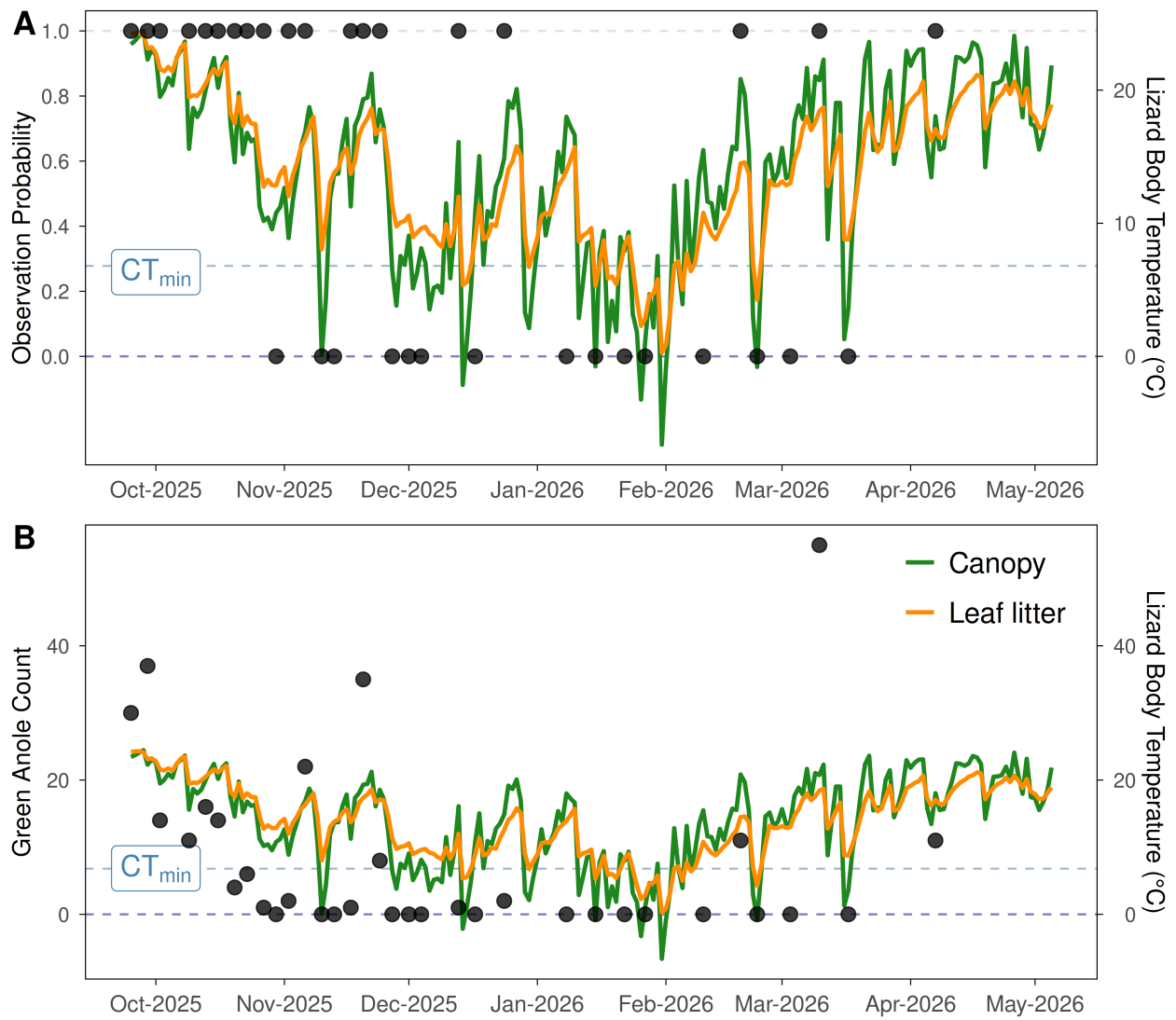
Figure S6. Presence (A) and number (B) of American green anoles ( Anolis carolinensis ) observed during our 34 night surveys between September 2025 and April 2026 in Atlanta, Georgia, USA (black points). Green and orange lines show the average operative temperature recorded by operative temperature models (OTMs) deployed in the canopy and in the leaf litter, respectively, between 1 and 2 hours after sunset on each day. The steel blue dashed line marks CT_{min} (6.8 °C, the lowest population-average CT_{min} across the species' range) and the dark blue dashed line 0 °C. Lizards disappeared from the vegetation as temperatures dropped in fall and winter, and reappeared on warm nights in winter and spring.
