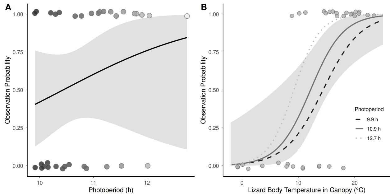
Figure S7. Photoperiod does not explain the decline in the probability of observing American green anoles ( Anolis carolinensis ) during our night surveys. (A) Predicted observation probability as a function of photoperiod at the average canopy operative temperature across surveys (13.1 °C). Points show the presence or absence of lizards in each survey, shaded by photoperiod (darker for shorter days). (B) Predicted observation probability as a function of canopy operative temperature at the shortest (9.9 h), average (10.9 h) and longest (12.7 h) photoperiods of our surveys. Lines show the predictions of a Bernoulli generalized linear model including canopy temperature, photoperiod and their interaction (Table S5), and shaded areas the 95% confidence intervals of the predictions (in B, at the average photoperiod only).
