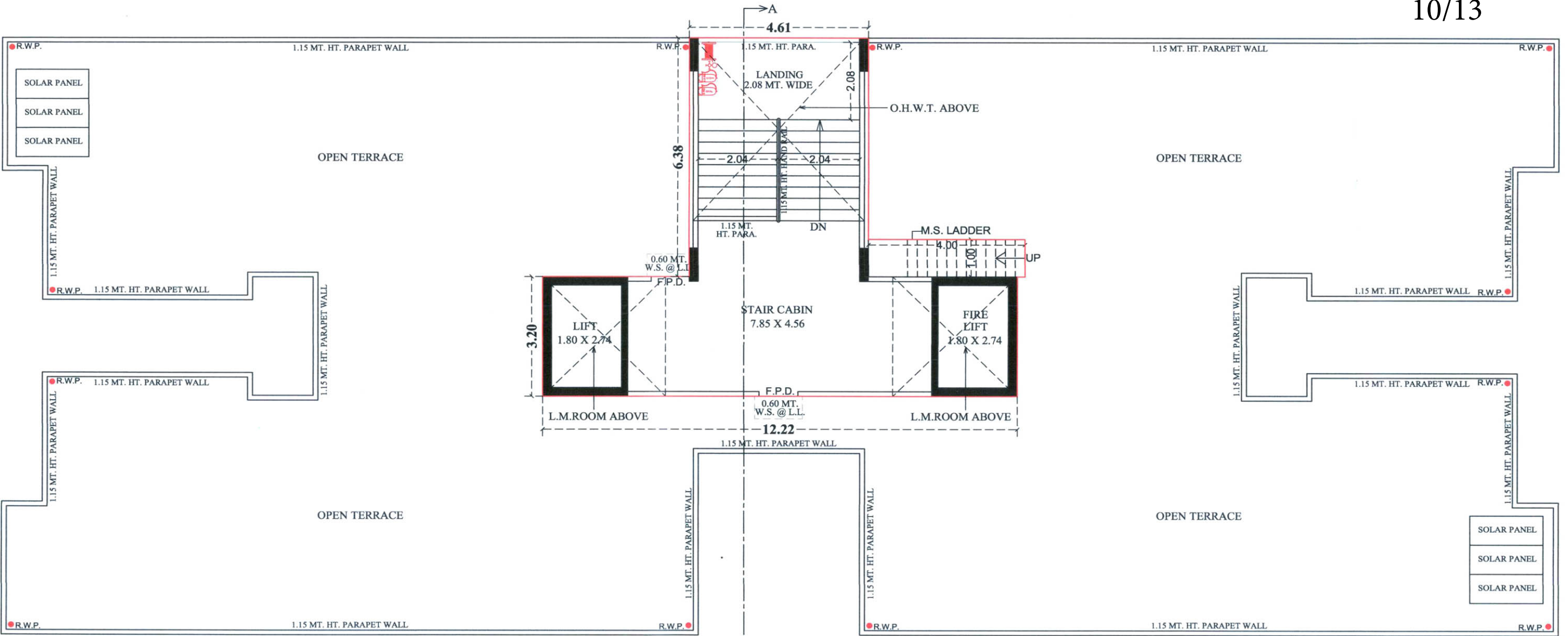
OPEN TERRACE PLAN (STAIR CABIN, LIFT MACH.ROOM&O.H.W.T.) NOTE :- ALL OUTER & INTERNAL WALL ARE OF 0.125 MT. TH. B/K WALL
