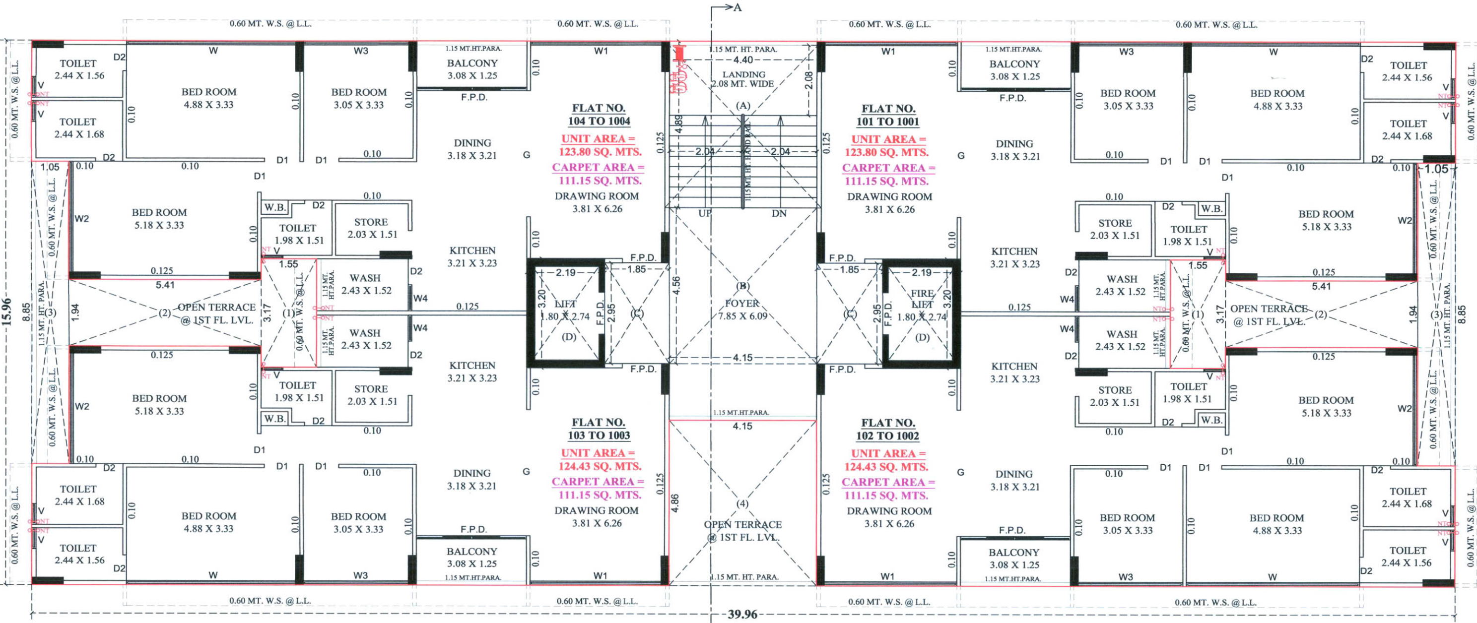
1ST FLOOR TO 10TH FLOOR PLAN NOTE :- ALL OUTER & INTERNAL WALL ARE OF 0.125 MT. TH. B/K WALL
