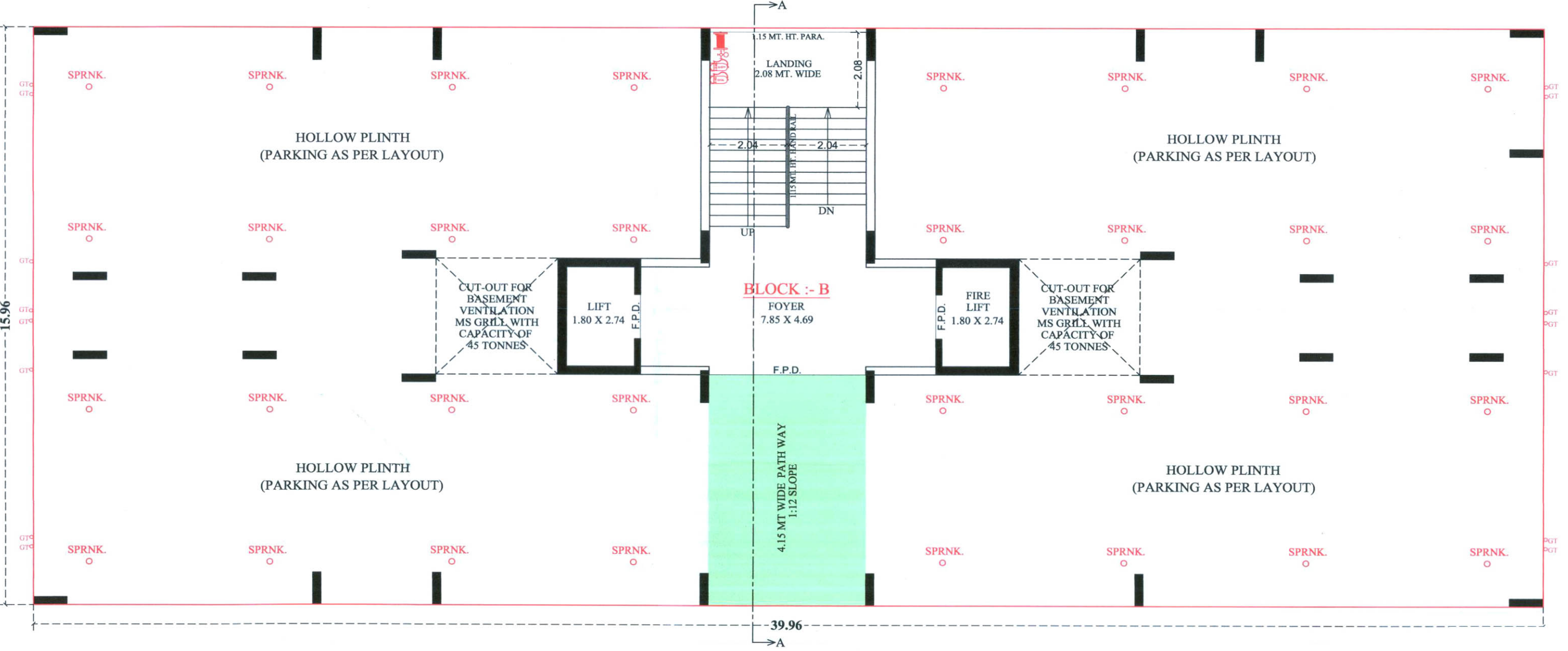
GROUND FLOOR PLAN (HOLLOW PLINTH) NOTE :- ALL OUTER & INTERNAL WALL ARE OF 0.125 MT. TH. B/K WALL
